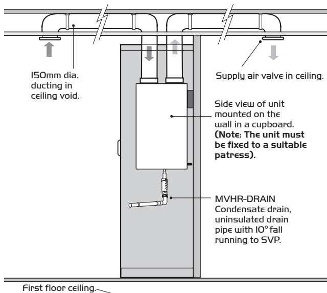
Figure 4. Typical example of a cupboard mounted unit on a patress using the bracket.
