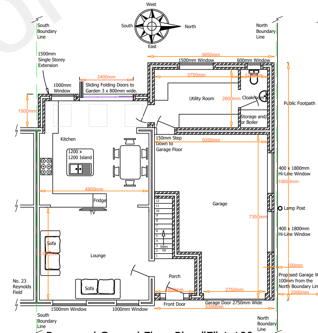
Proposed Ground Floor Plan "E" 1:100
