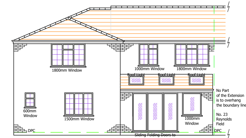
Proposed Rear (West) Elevation 1:100
