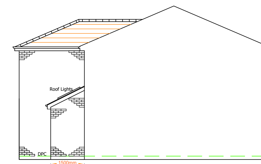
Proposed Side (South) Elevation 1:100
