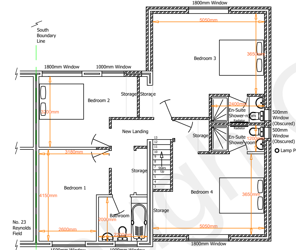
Proposed First Floor Plan "E" 1:100
