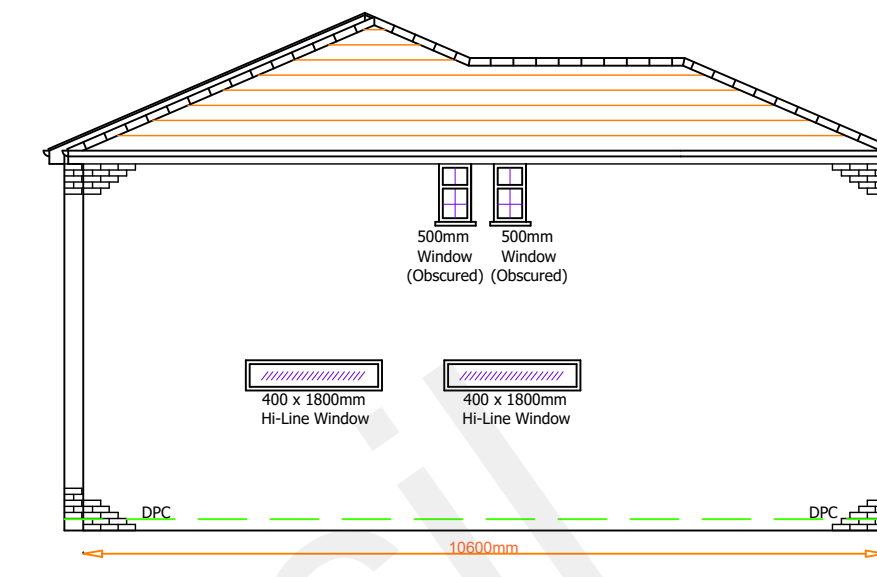
Proposed Side (North) Elevation 1:100
