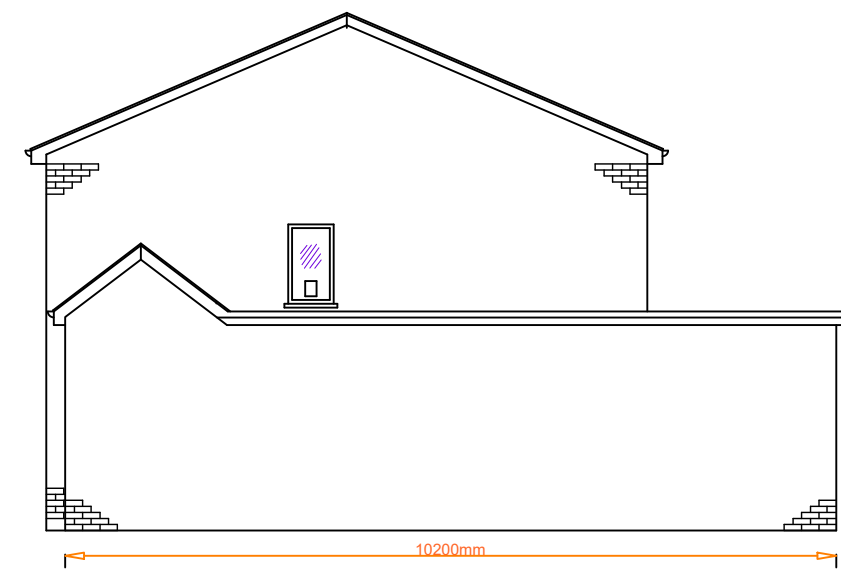
Existing Side (North) Elevation 1:100
