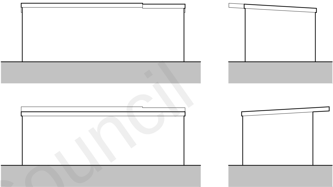
Existing Stables 01 Elevations 1:100
