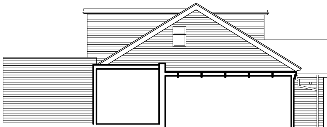
South Elevation
