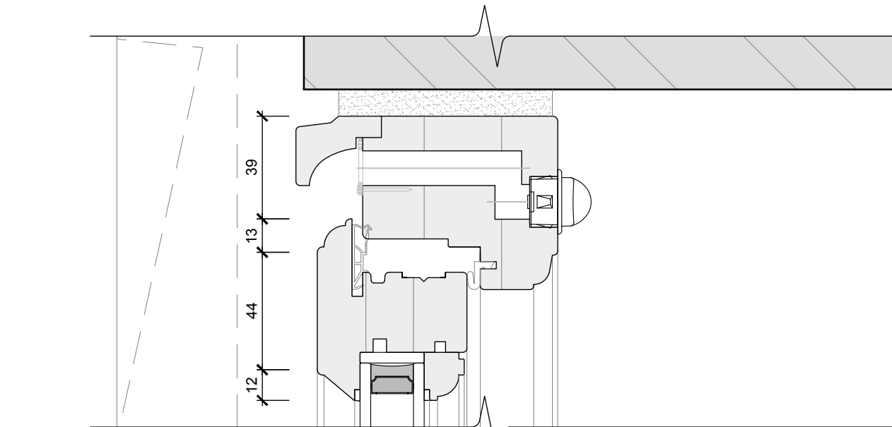
Proposed Head Detail 1:2
