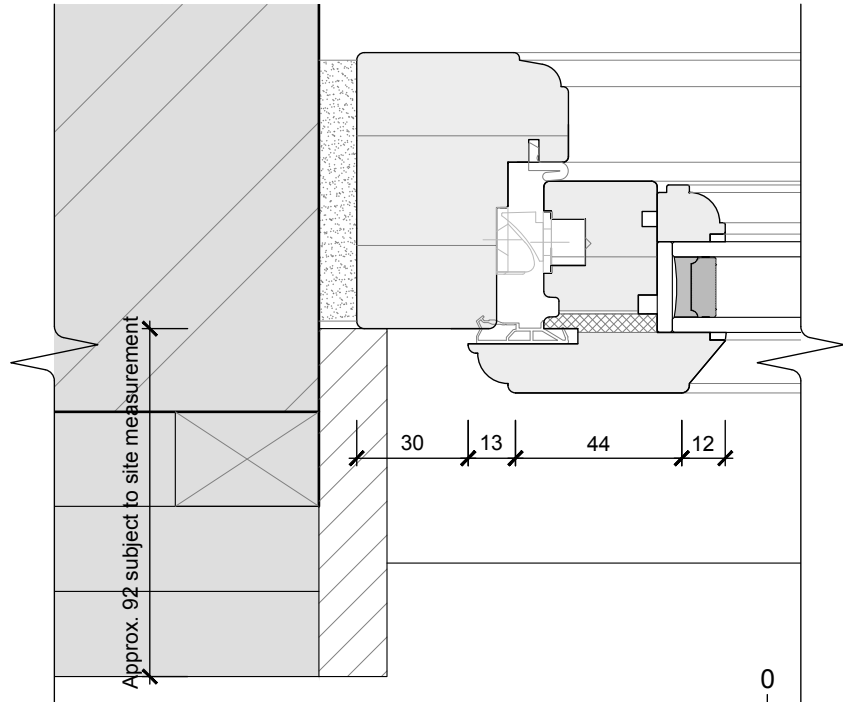
Proposed Jamb Detail 1:2
