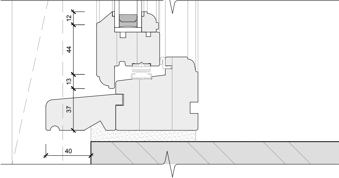
Proposed Cill Detail 1:2
