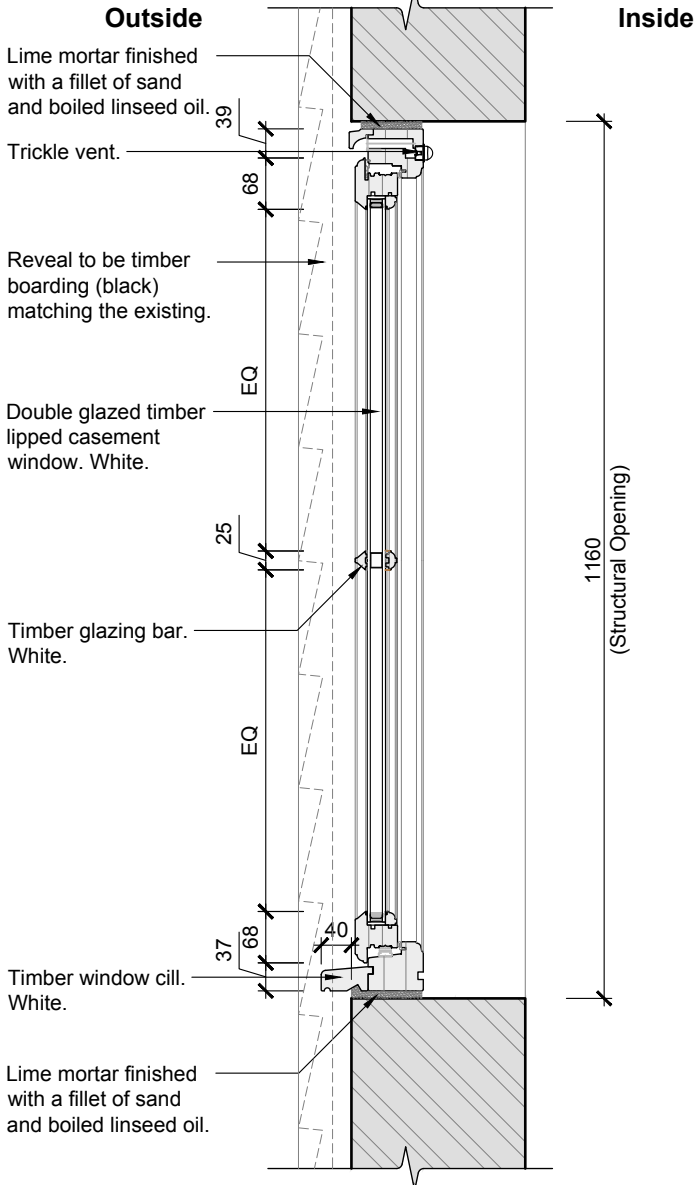
Proposed Section 1:10
