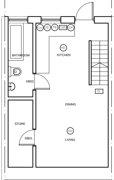
PROPOSED LOWER GROUND FLOOR PLAN
