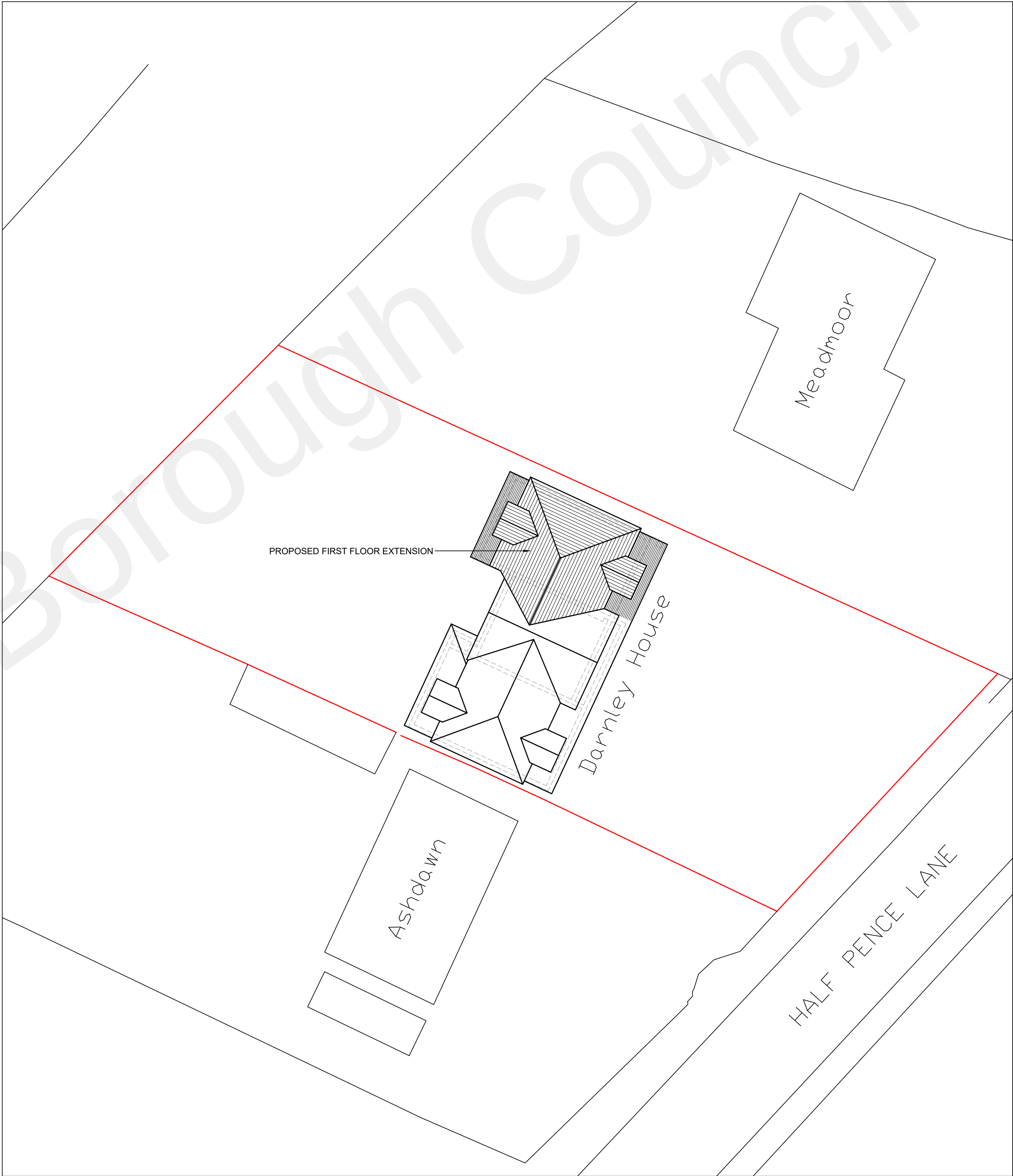
BLOCK PLAN AS PROPOSED (1:200)
