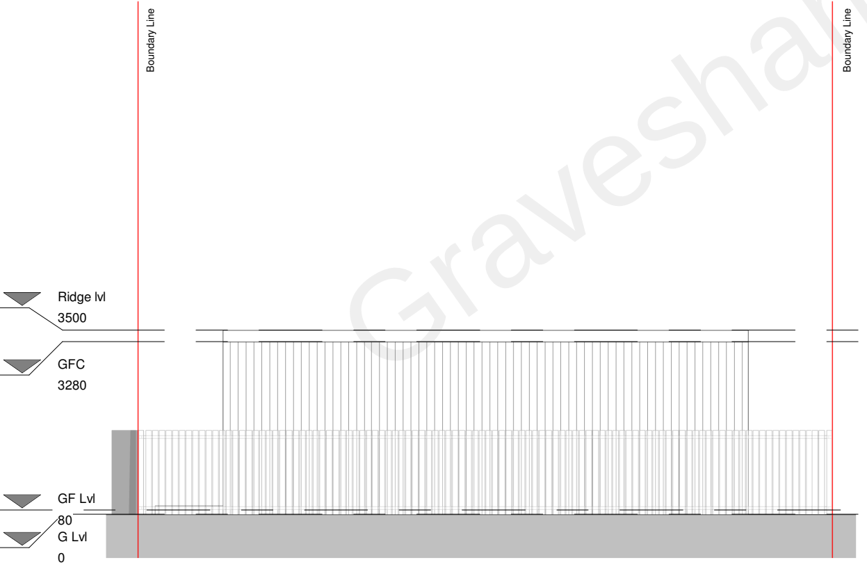
Rear elevation
