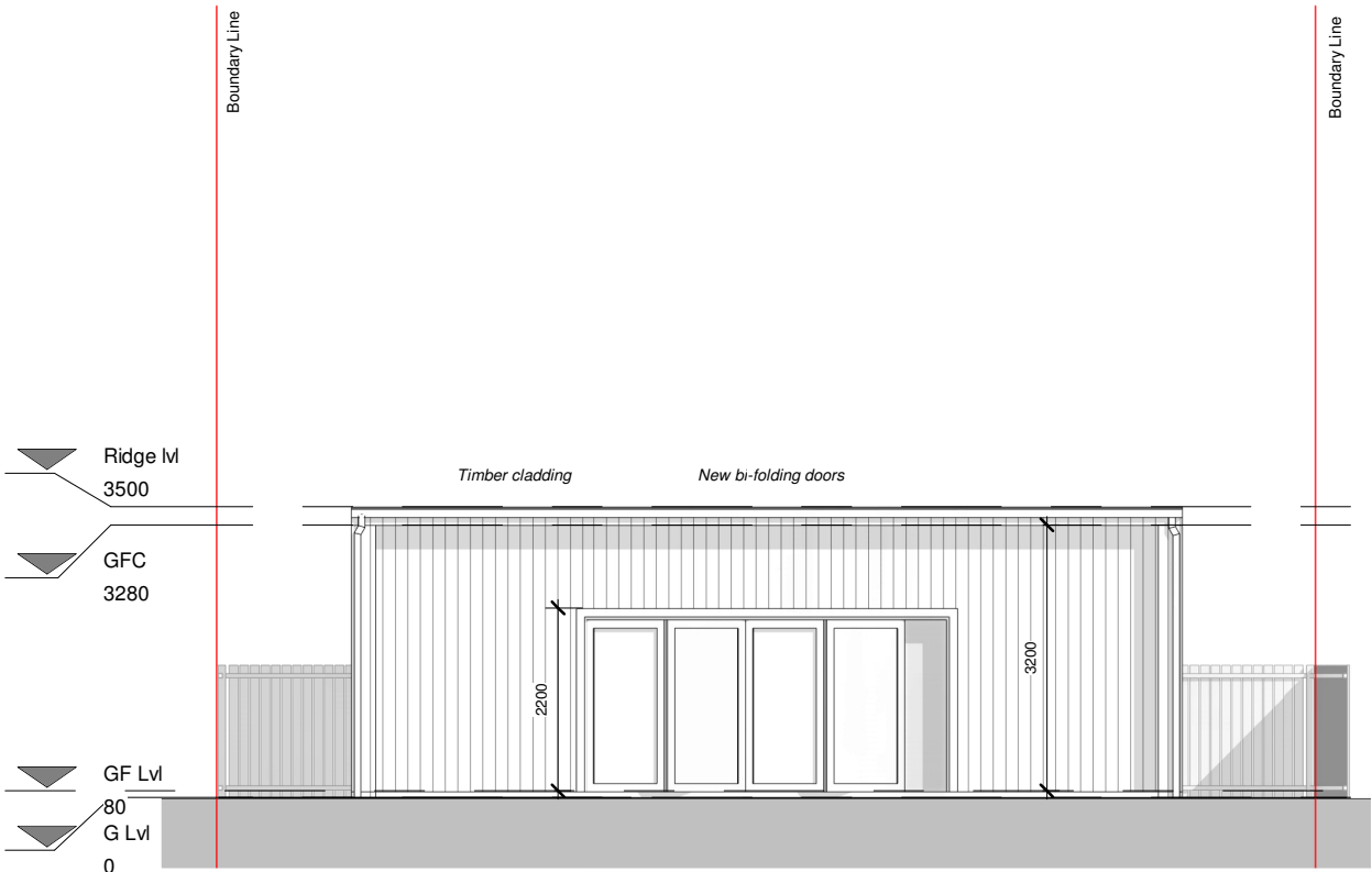
Front elevation
