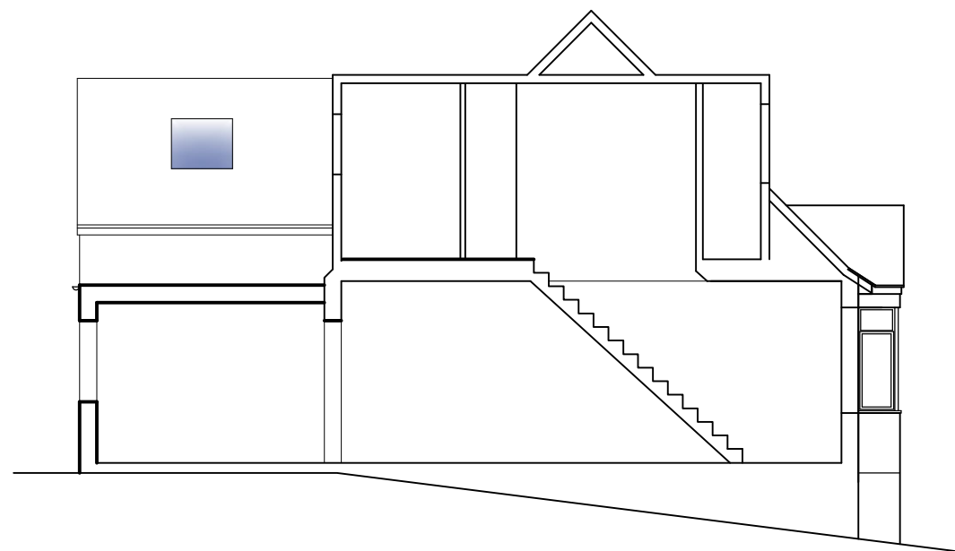
SIDE SECTIONAL ELEVATION
