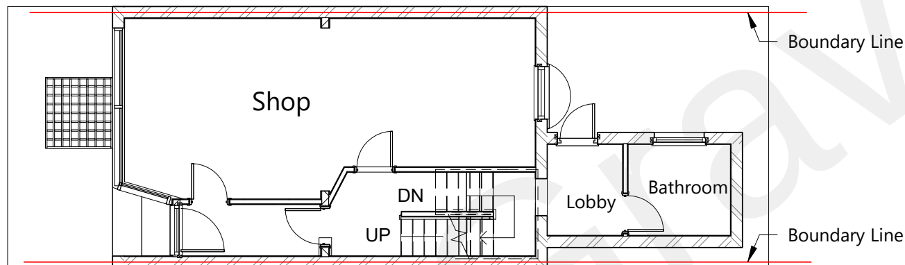
Existing Groundfloor Layout
