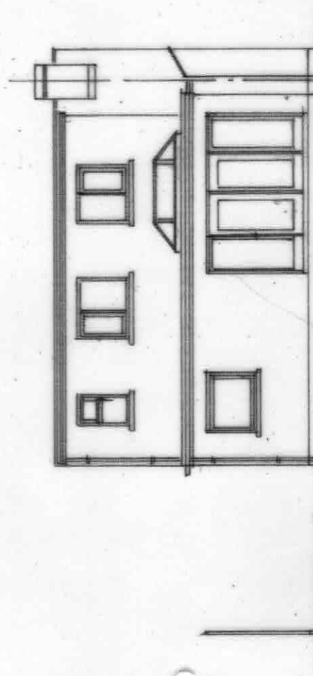
Rear Elevation
