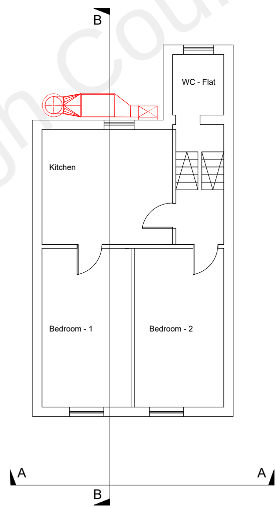
RETROSPECTIVE FIRST FLOOR PLAN
