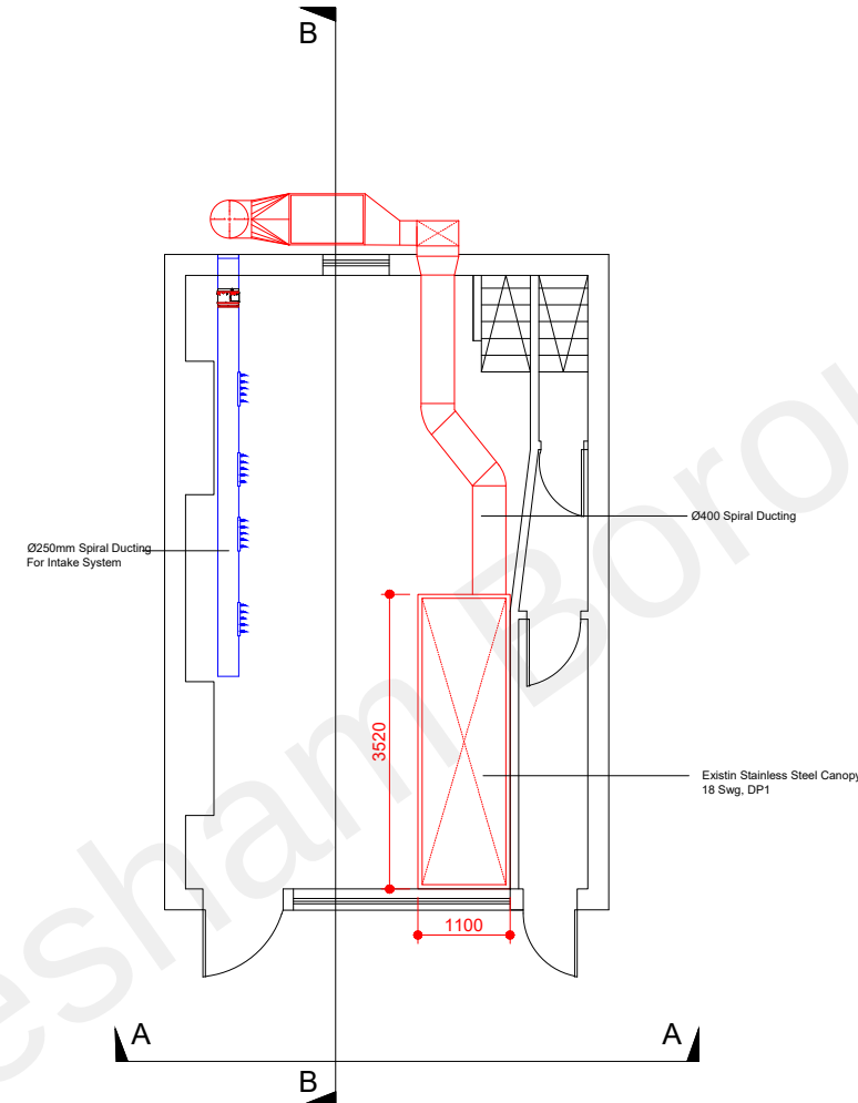
RETROSPECTIVE GROUND FLOOR PLAN
