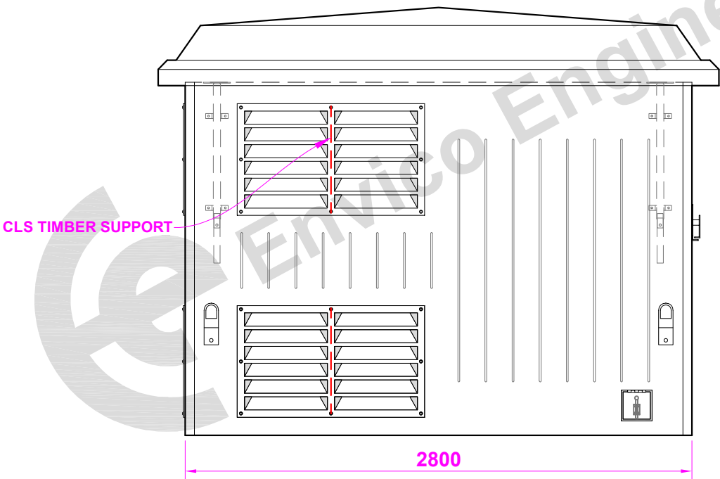
Elevation (B) (l/h side)
