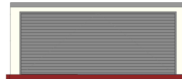
③ Front Elevation-Proposed 1 : 100
