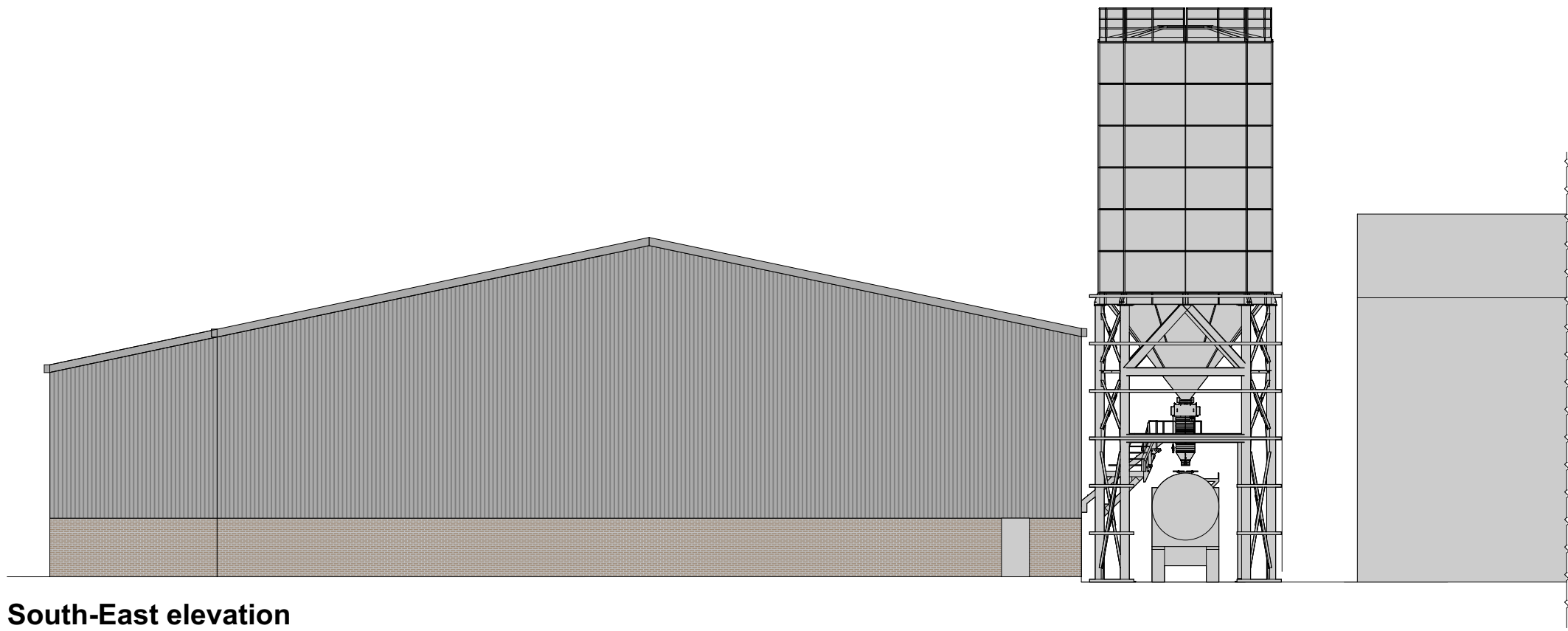
South-East elevation
