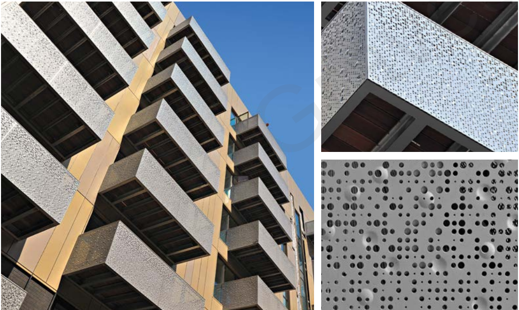
Project: Pembury Circus, London Sector: Residential Architect: Fraser Brown McKenna Finish: Polyester powder coated steel
