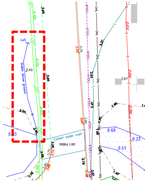
Figure 7: Extract from CEN26807 showing water main.
