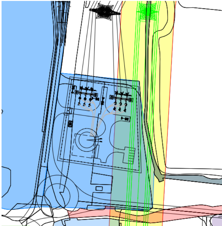
Figure 2: Tilbury site proposed layout and location.
