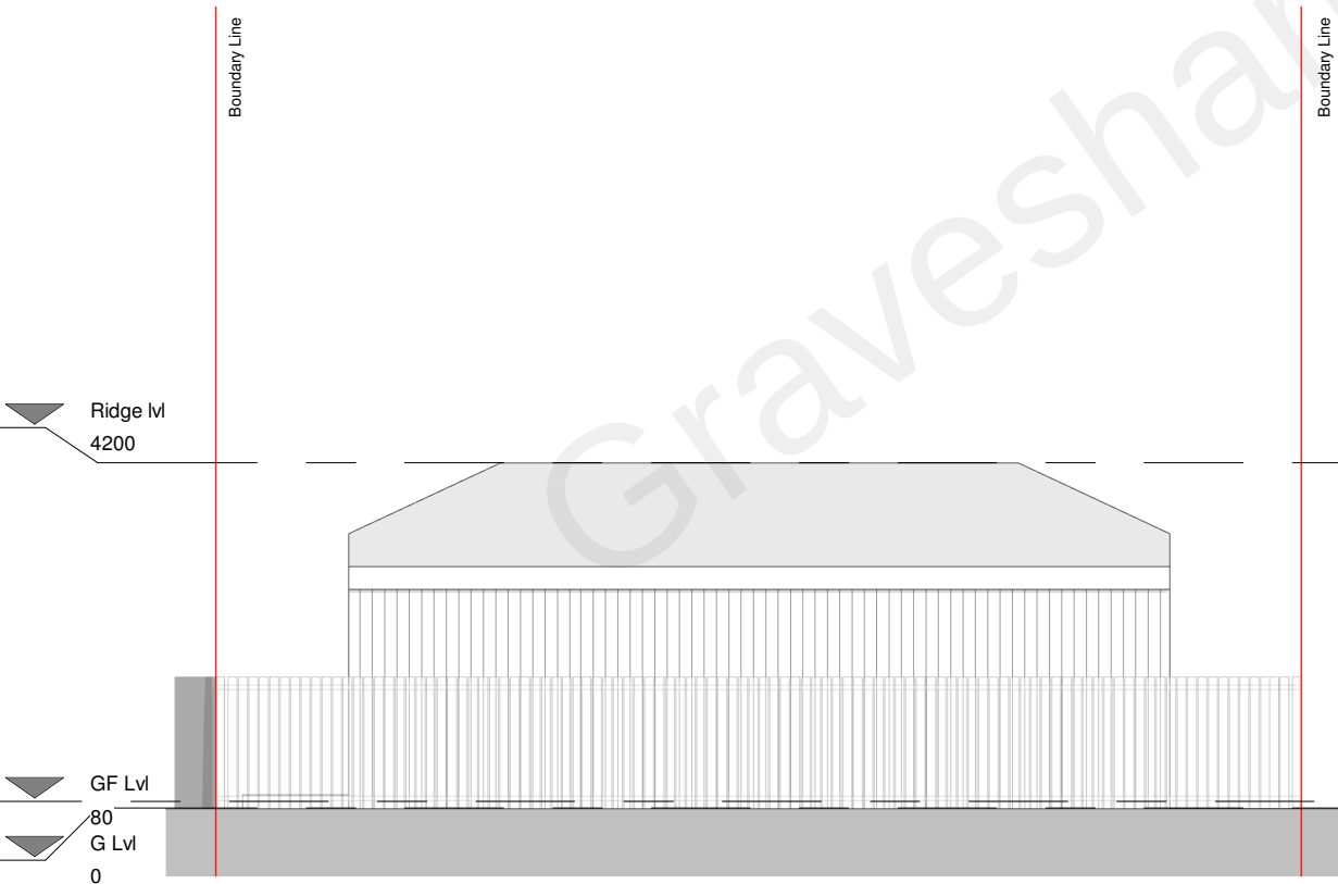
Rear elevation
