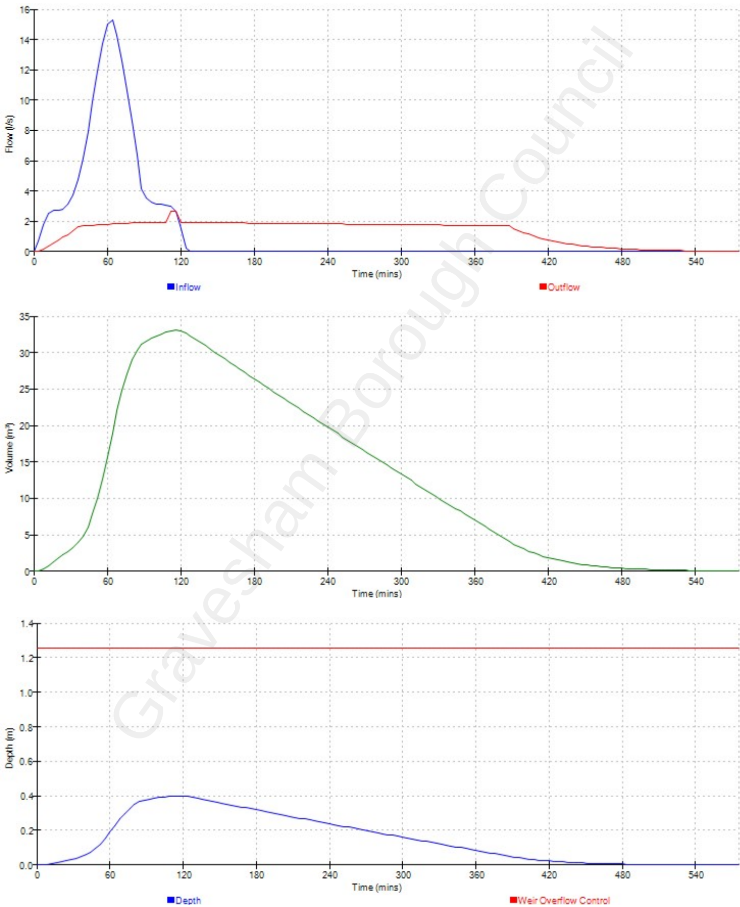
Event: Input Hydrograph
