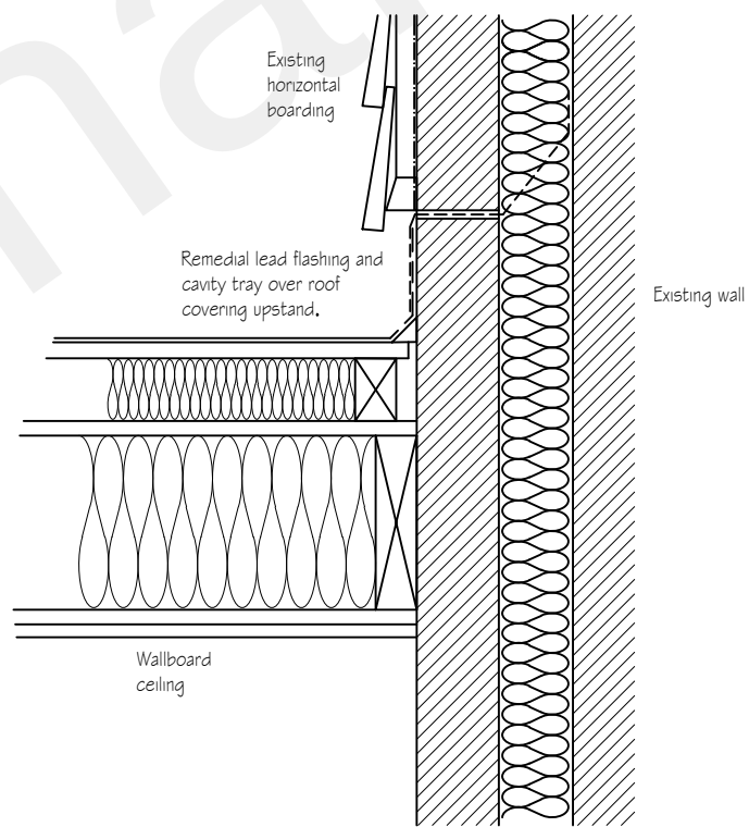
Flat roof abutment Scale 1:10
