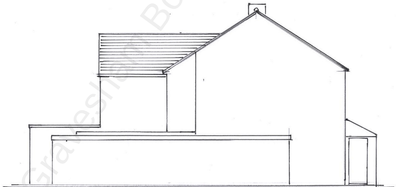
PROPOSED SIDE ELEVATION -1:50 - VIEWED SOUTHERLY
