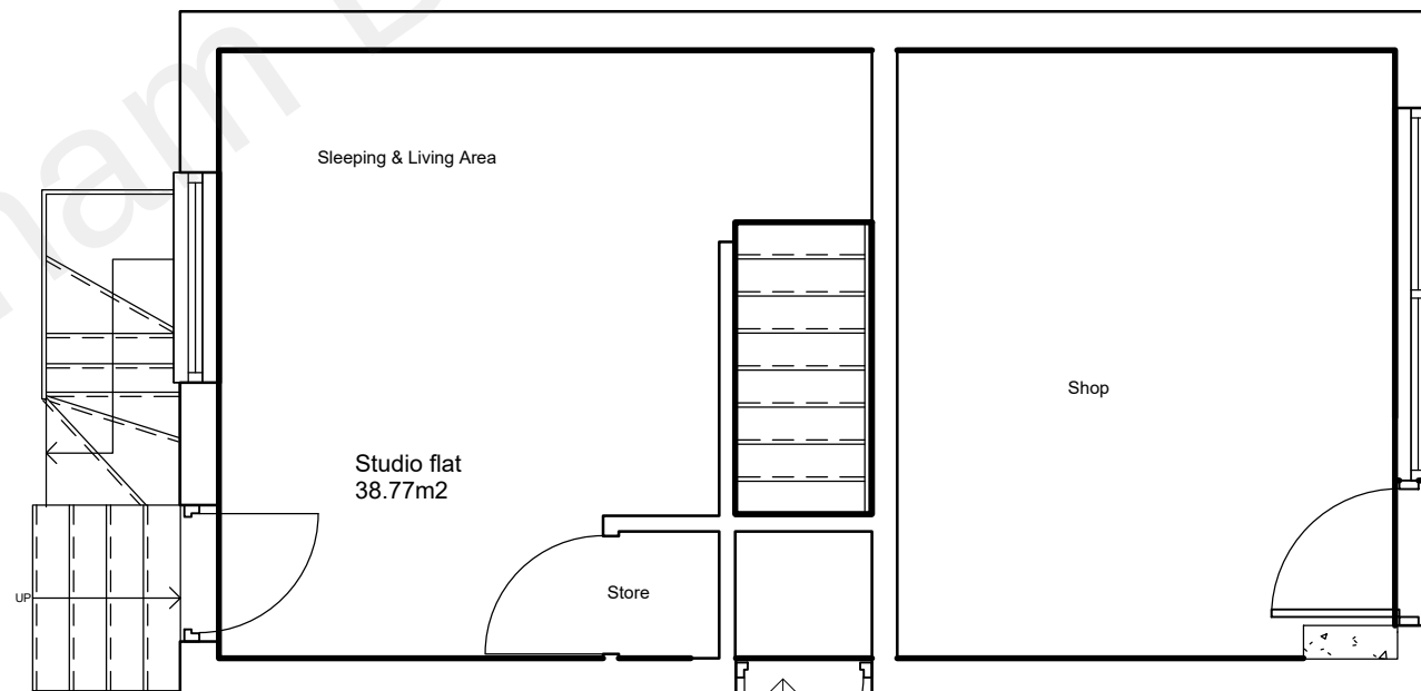
01. GF Proposed 1 : 50
