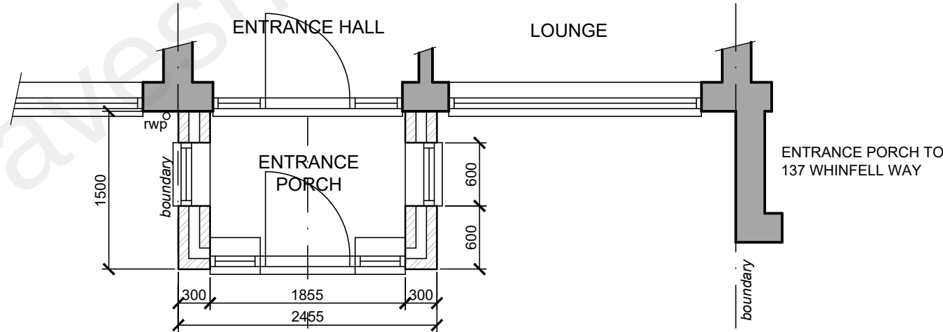
PART GROUND FLOOR PLAN (1:50)
