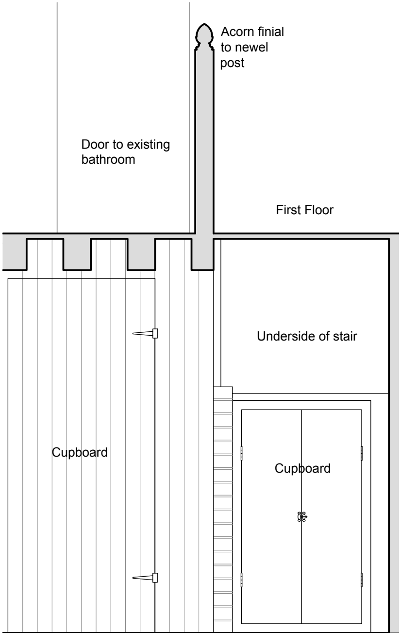
Existing C19 Staircase Rear Interior Elevation (Elev. 02)
