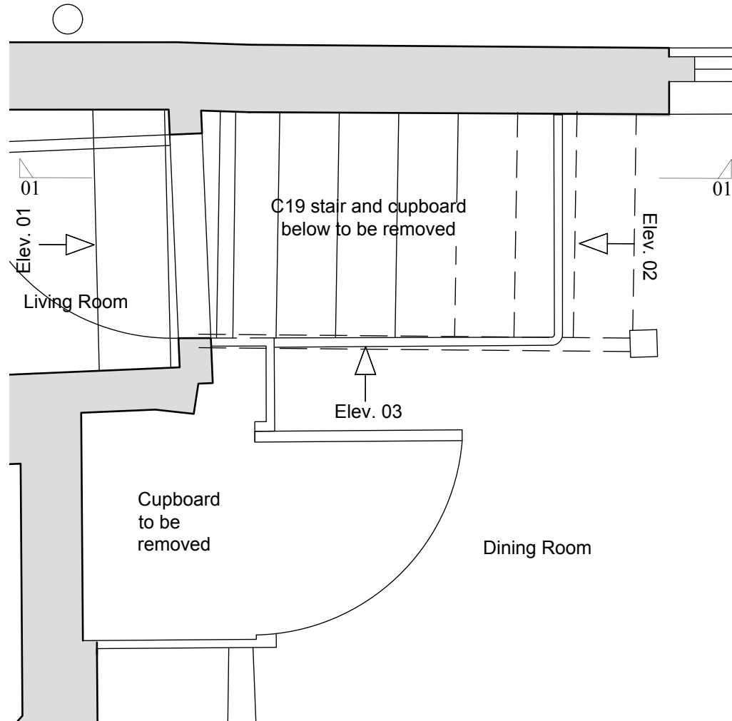
Existing C19 Staircase Plan
