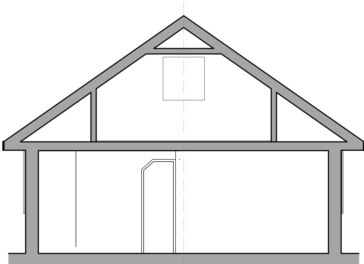
SECTION A-A (1:50)
