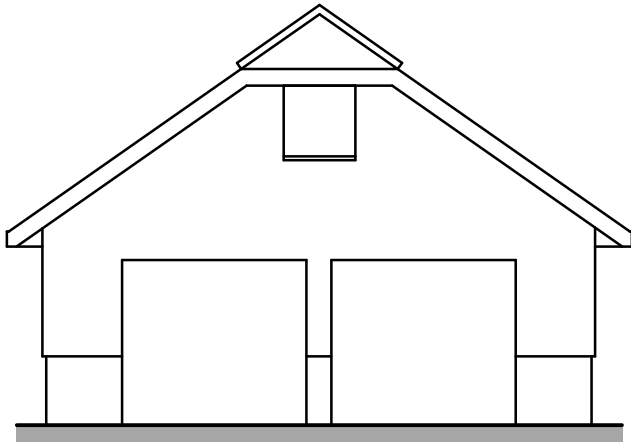
FRONT ELEVATION (1:100)
