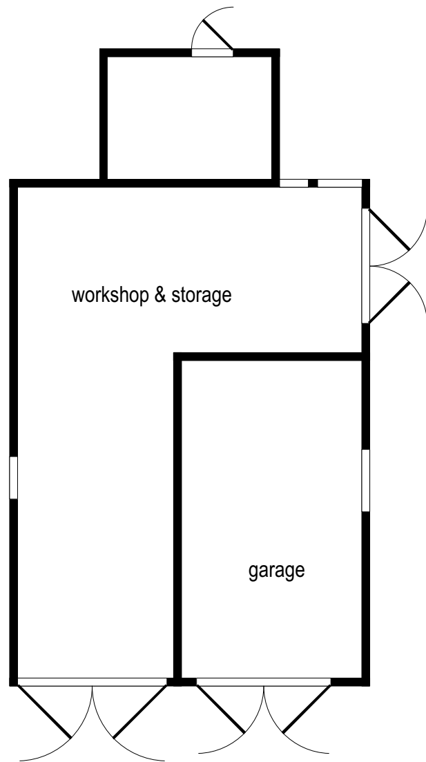
existing ground plan - 70 sqm.
