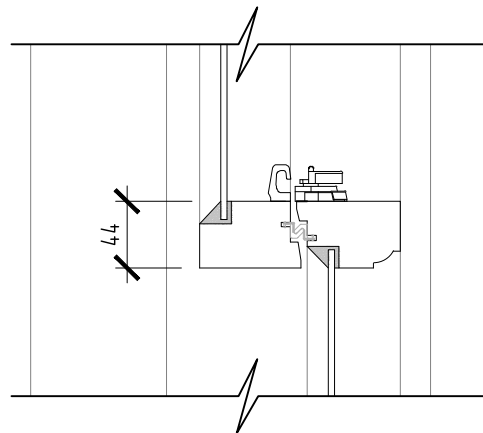
Single glazed timber box sash head detail
