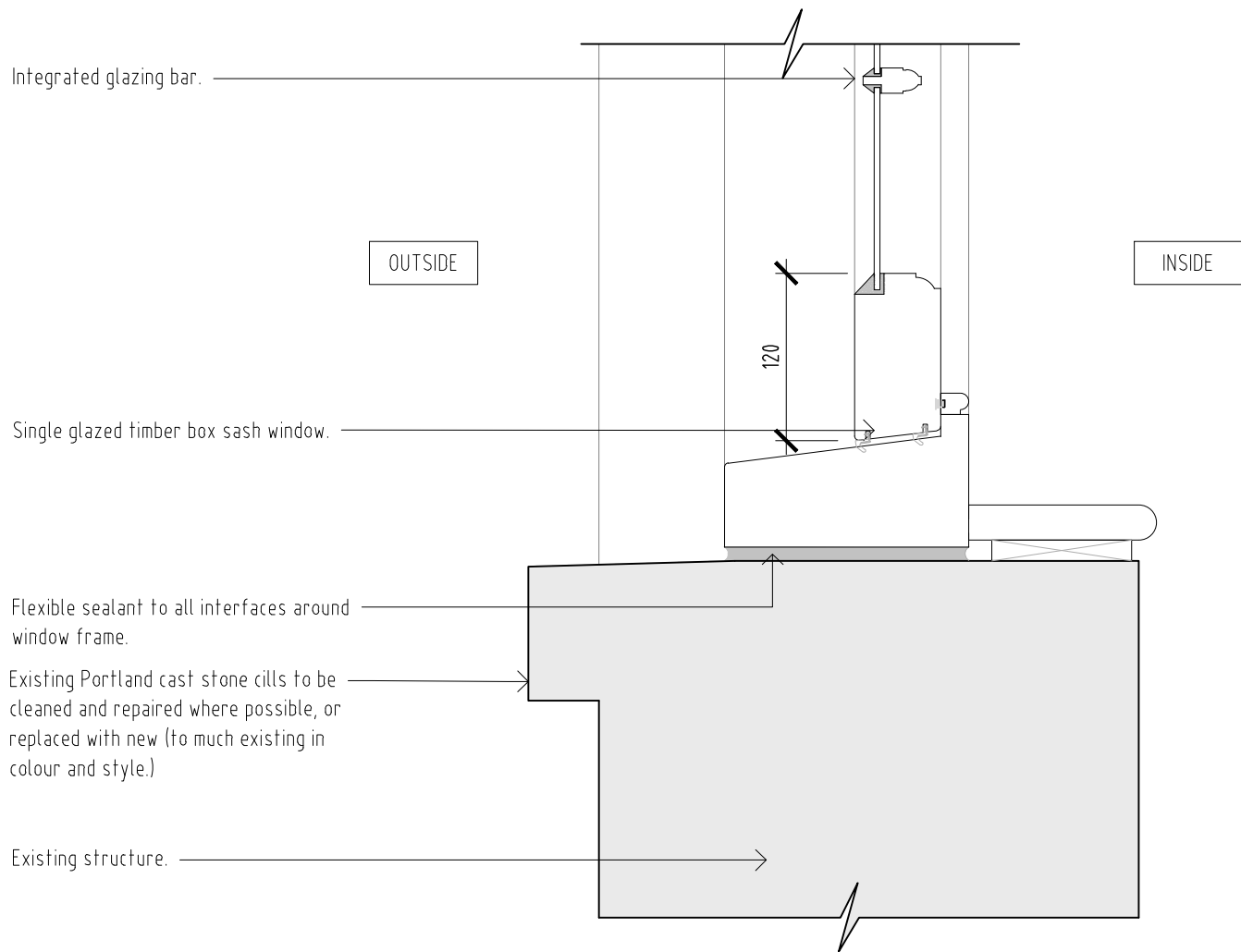
Single glazed timber box sash cill detail
