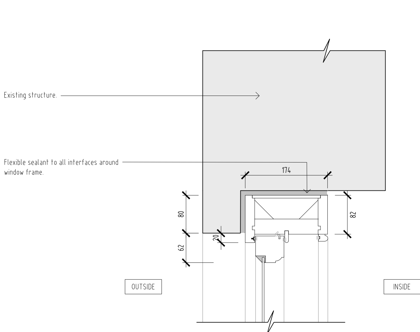
Single glazed timber box sash head detail
