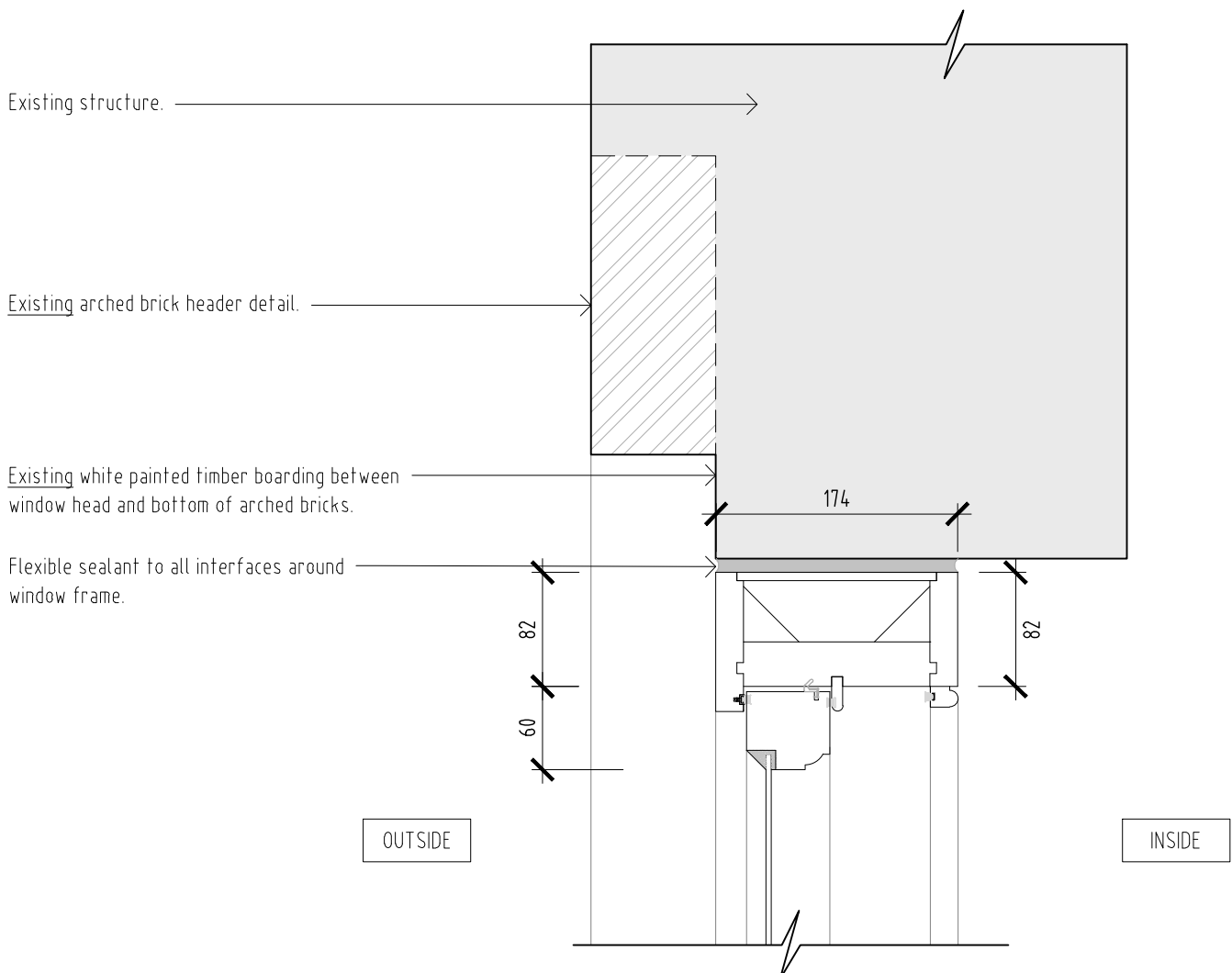
Single glazed timber box sash cill head detail w/existing arched header
