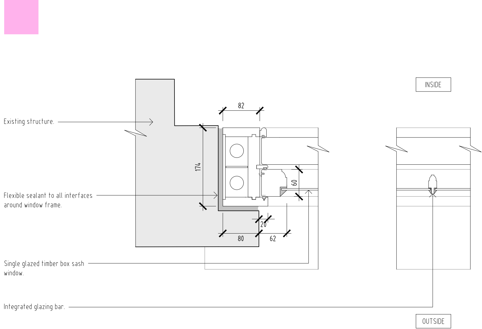
Single glazed timber box sash cill detail
