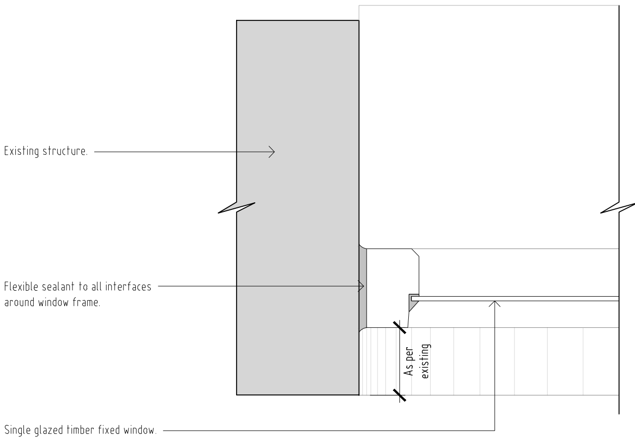
Single glazed timber fixed window jamb detail
