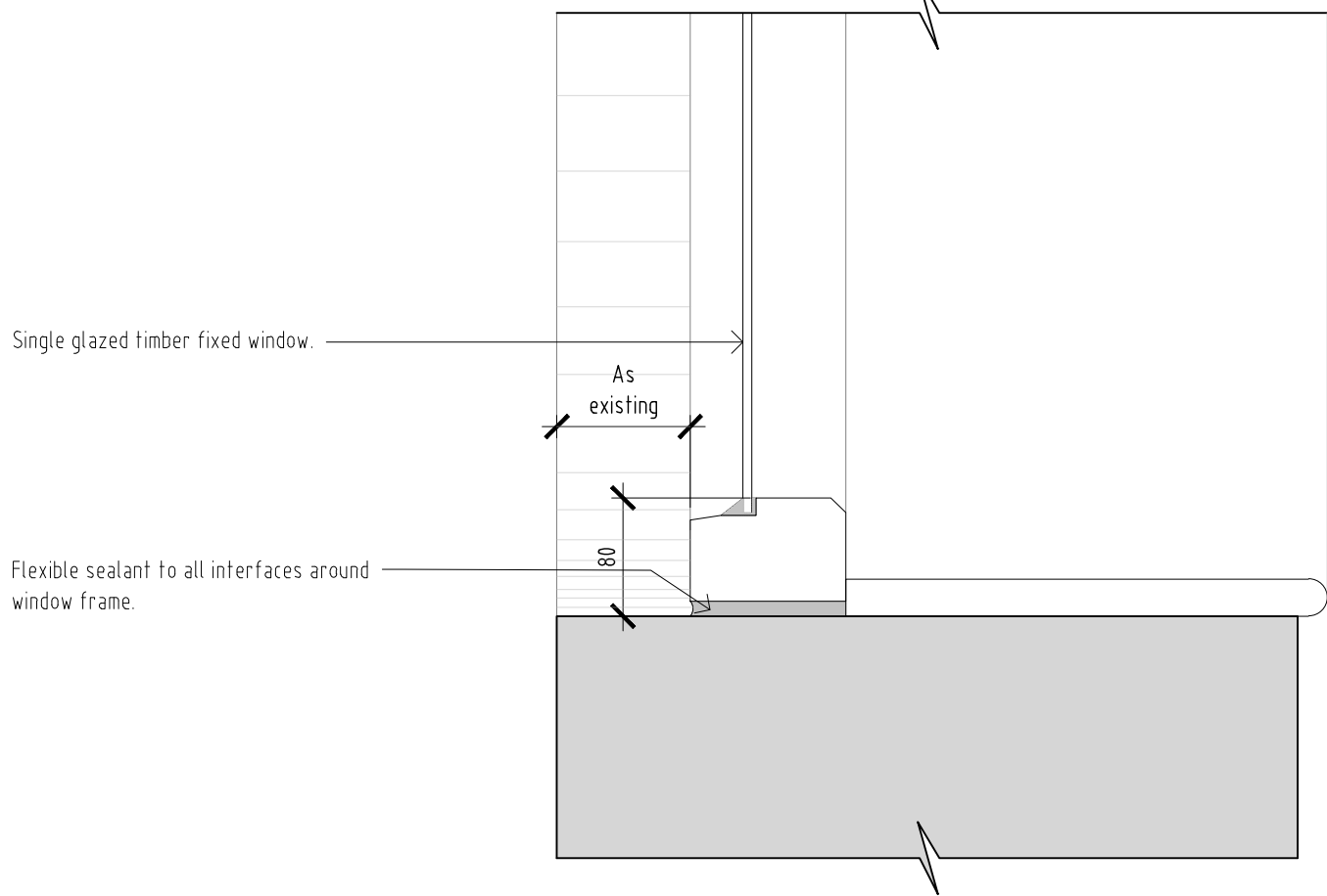
Single glazed timber fixed window cill detail
