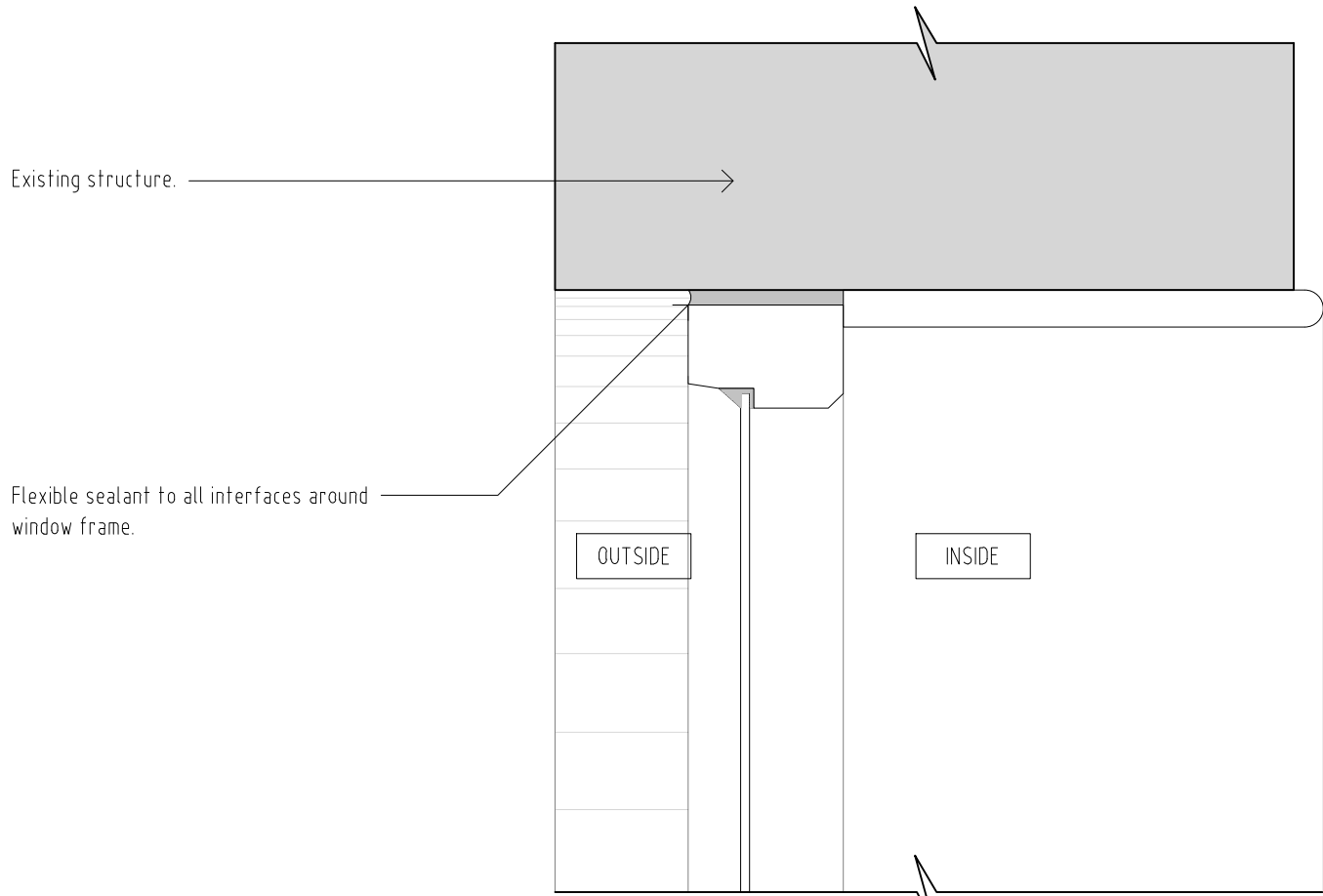
Single glazed timber fixed window head detail
