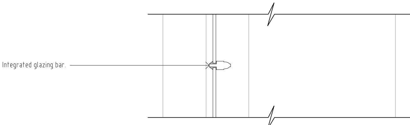
Single glazed timber French doors transom detail
