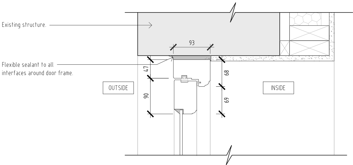
Single glazed timber French doors head detail
