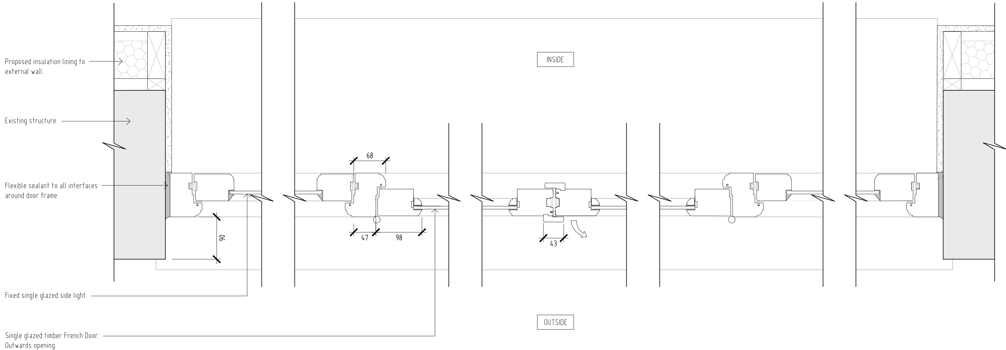
Single glazed timber French doors with sidelights jamb detail
