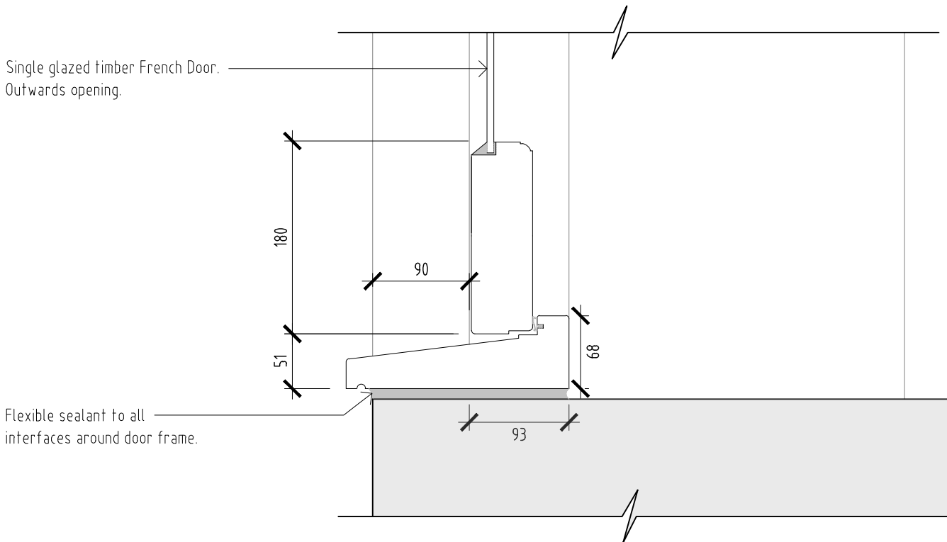
Single glazed timber French doors cill detail
