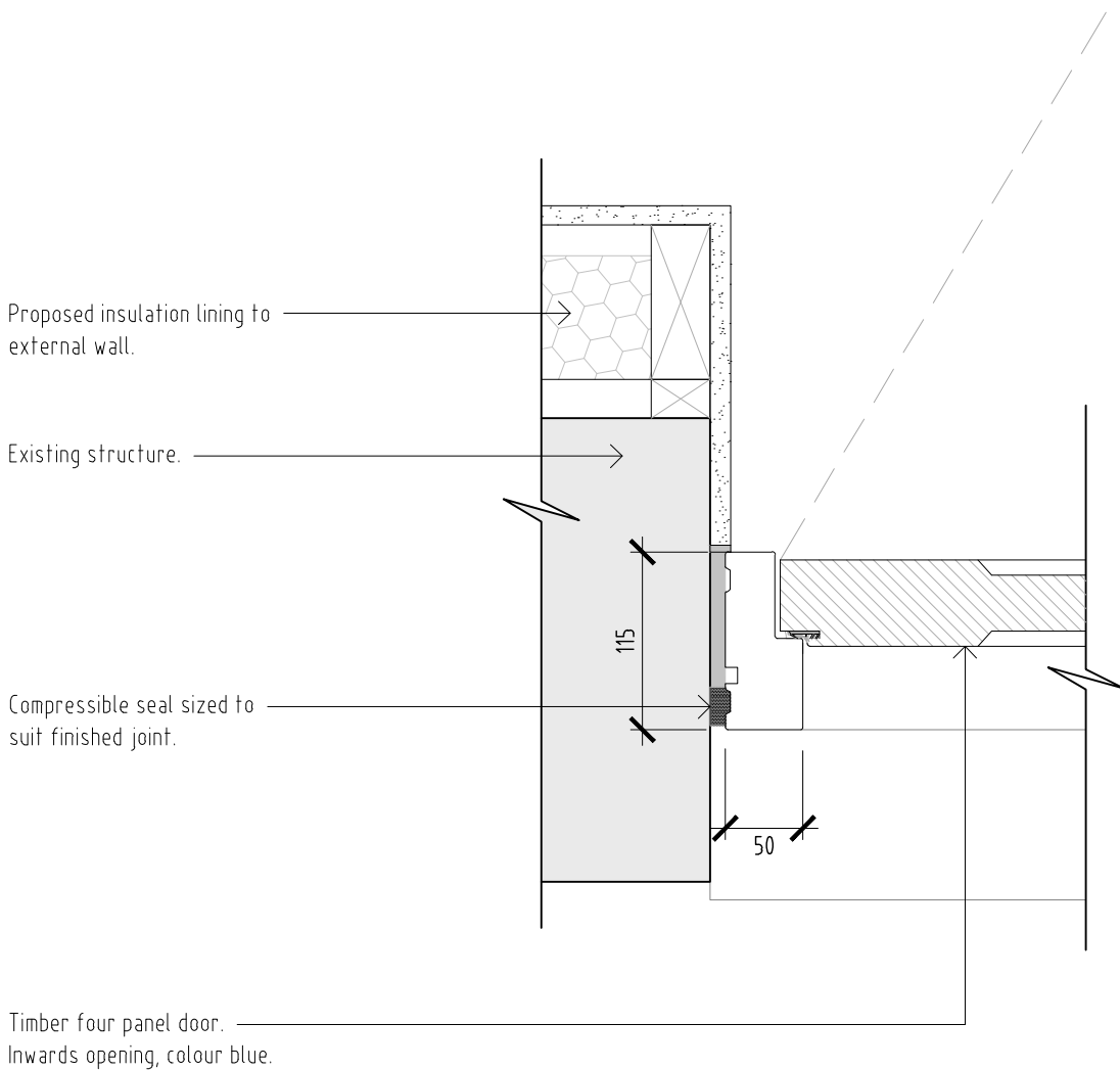
Timber front door jamb detail
