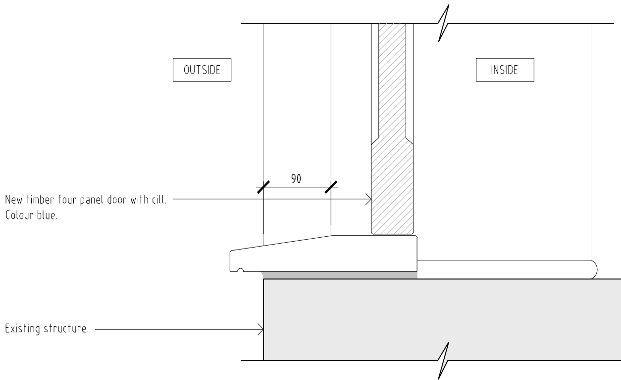
Timber front door cill detail
