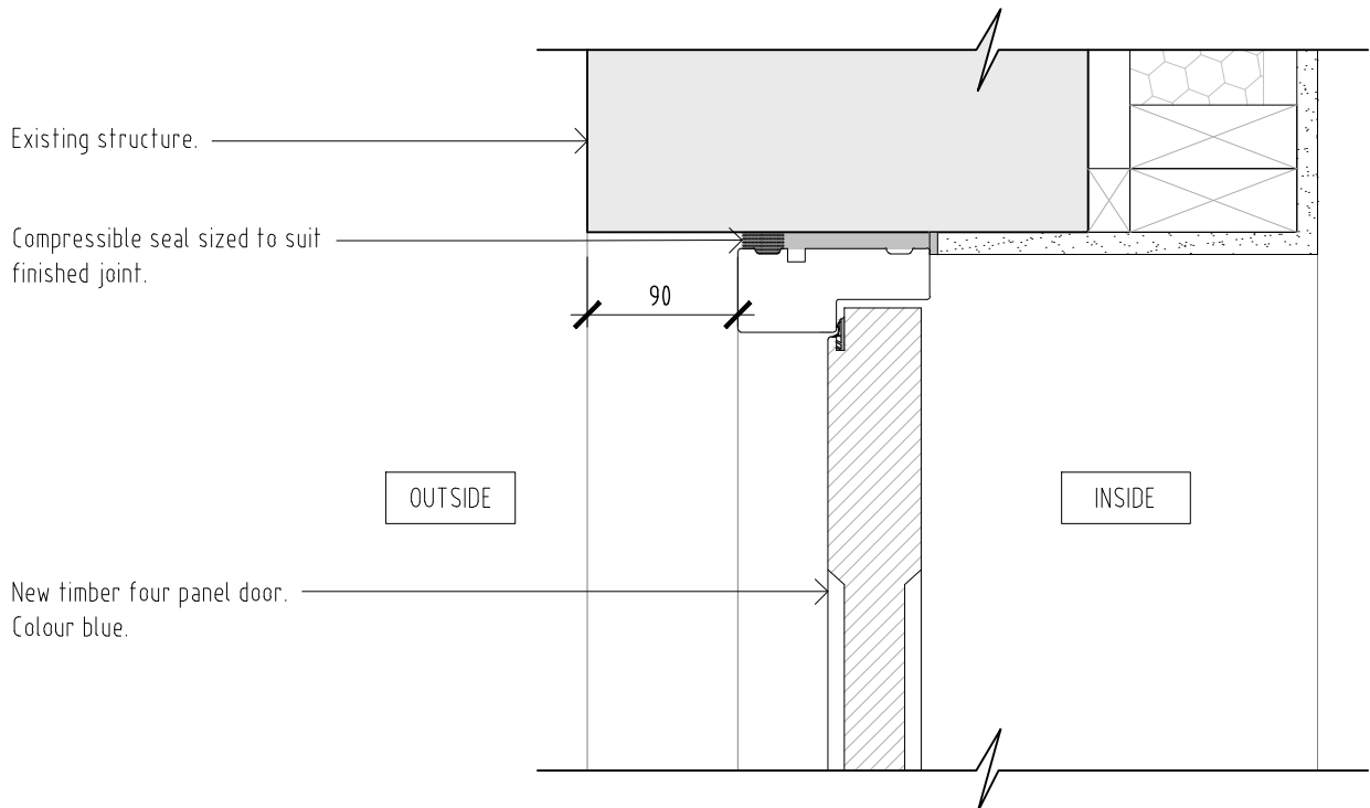
Timber front door head detail
