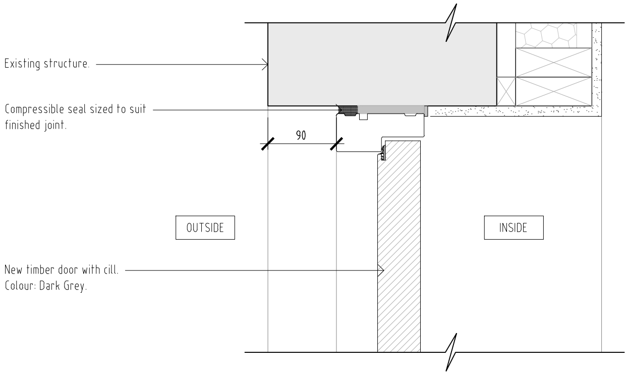
Modern style timber door head detail
