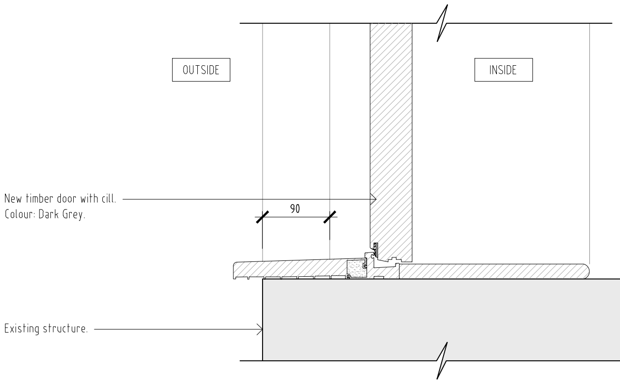
Modern style timber door cill detail
