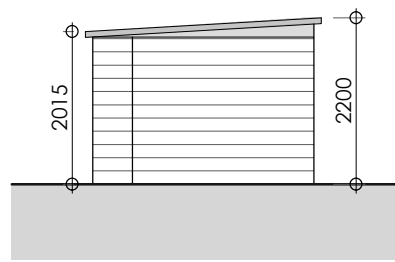
STRUCTURE B - LEFT FLANK
