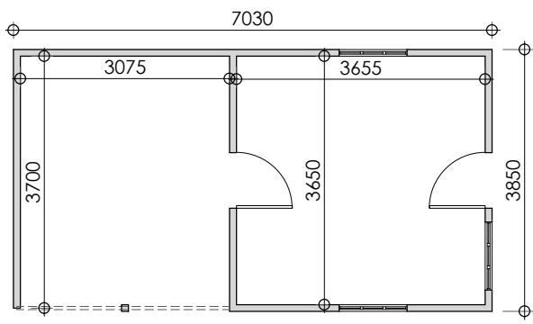
STRUCTURE C - FLOOR PLAN
