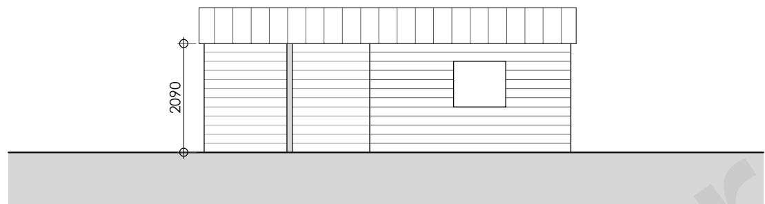
STRUCTURE C - FRONT ELEVATION
