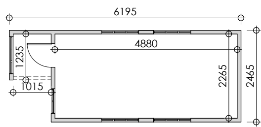
STRUCTURE D - FLOOR PLAN
