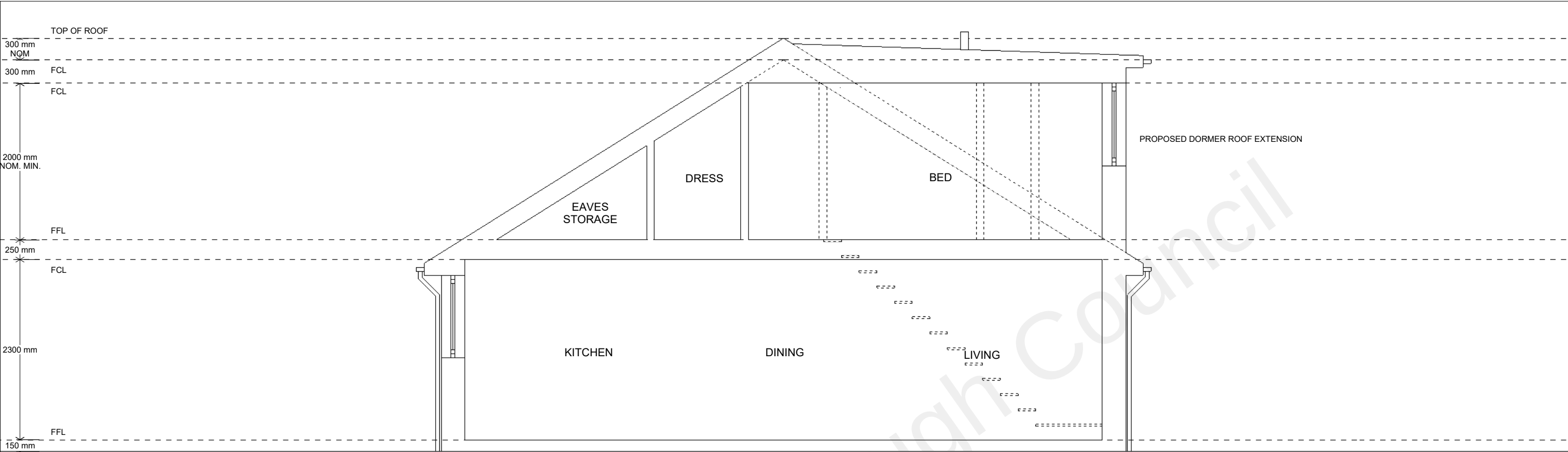
SECTION CC
