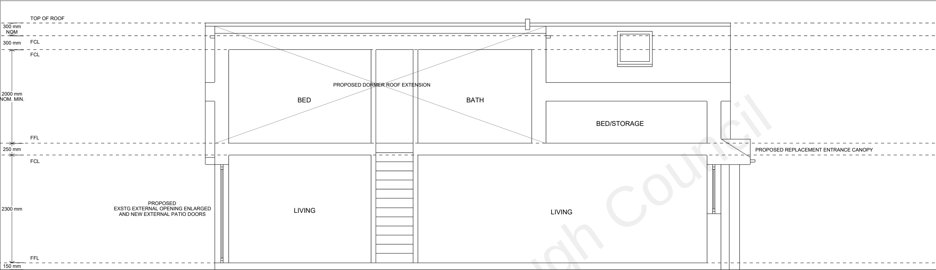
SECTION AA
