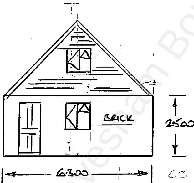
REAR ELEVATION
