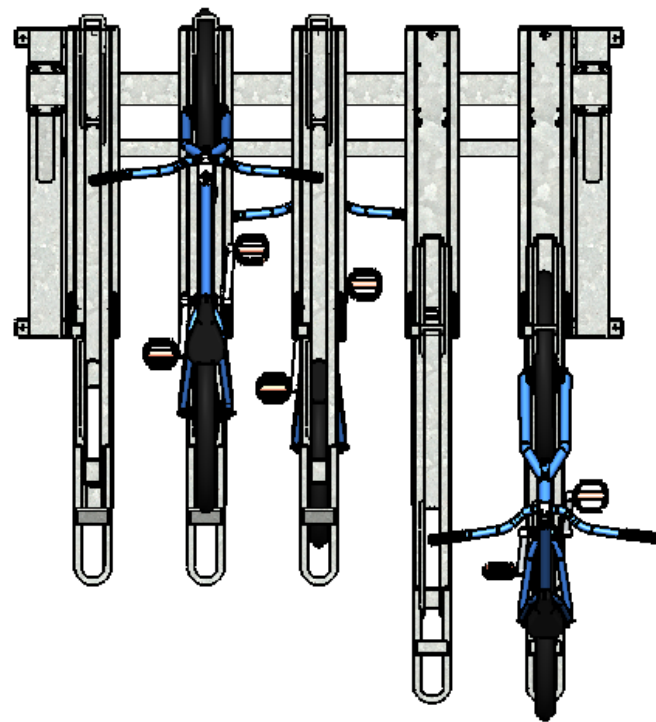
PLAN VIEW WITH BICYCLES
