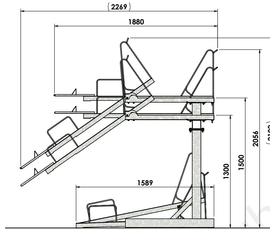
SIDE ELVEATION WITHOUT BICYCLES
