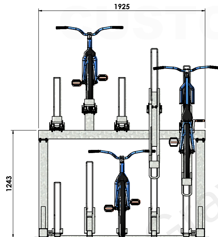
FRONT ELVEATION WITH BICYCLES
