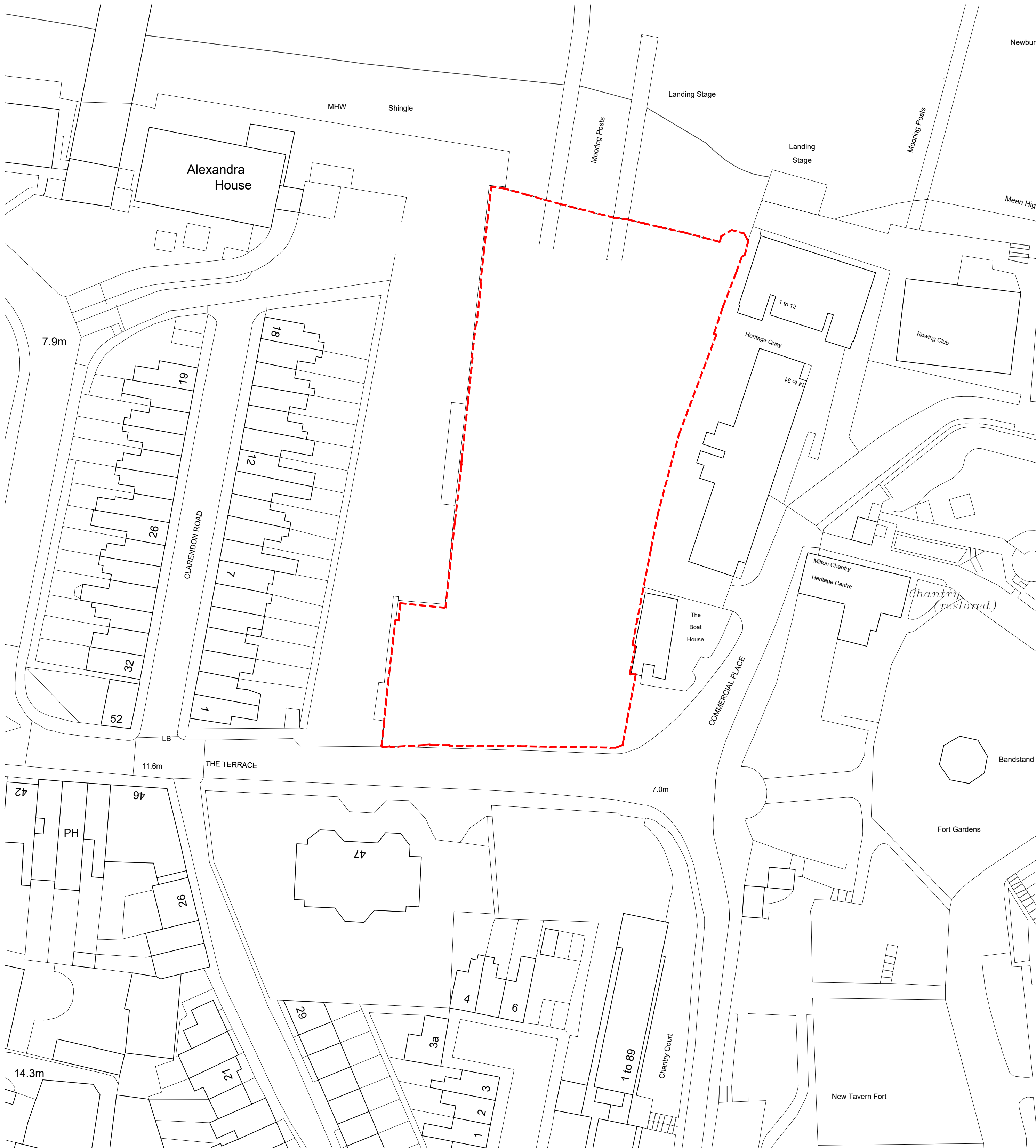
Site Block Plan 1:500
