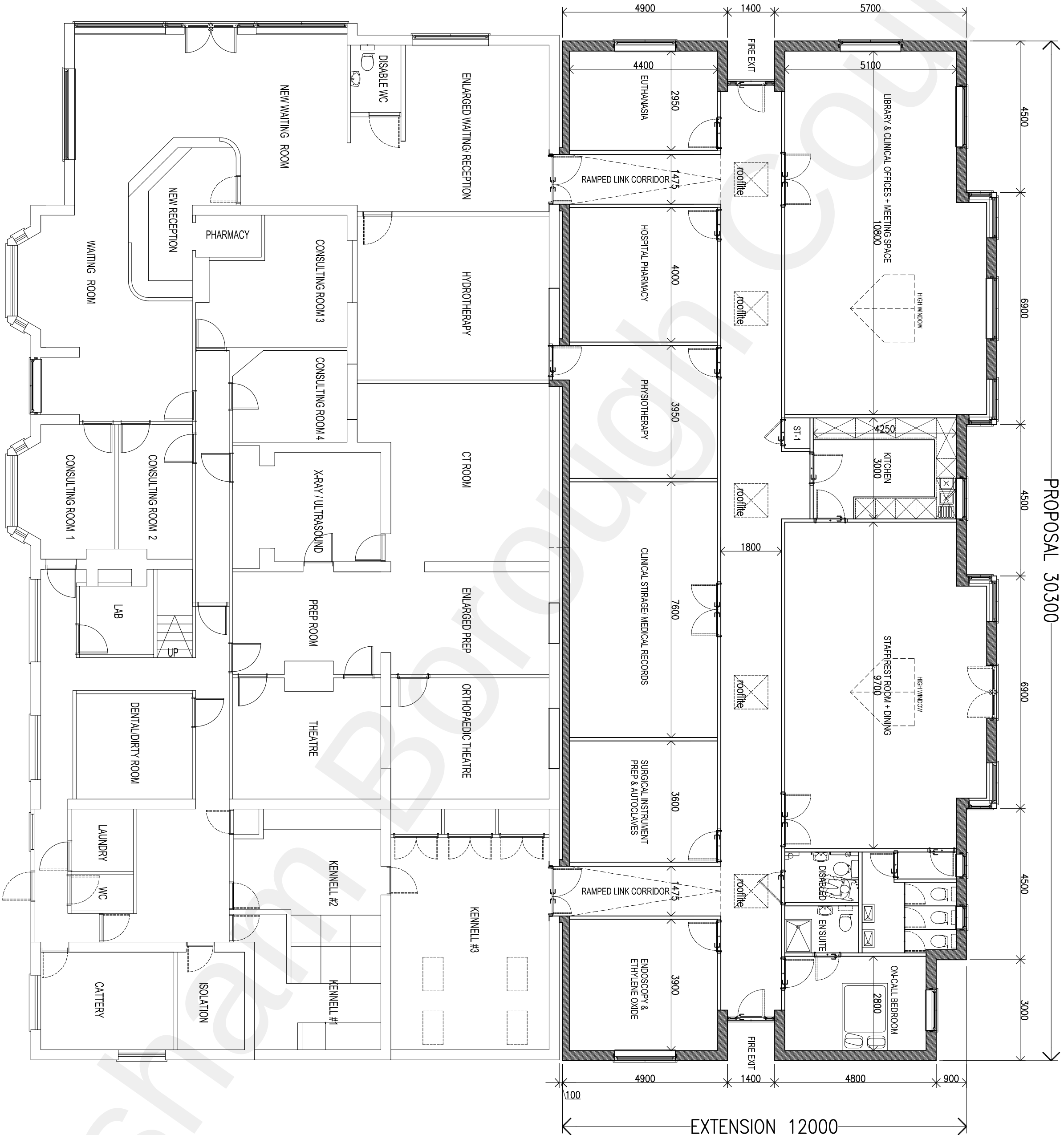
PROPOSED GROUND FLOOR PLAN 370m2 GROSS EXTERNAL
