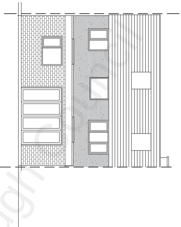
Rear Elevation
