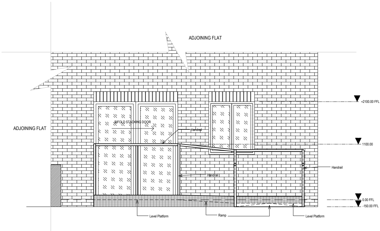
PROPOSED ELEVATION/SECTION 1:50
