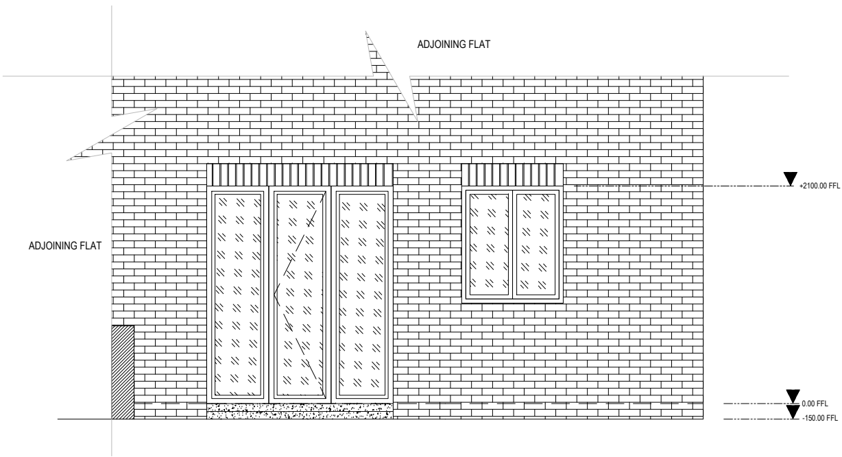
EXISTING ELEVATION 1:50
