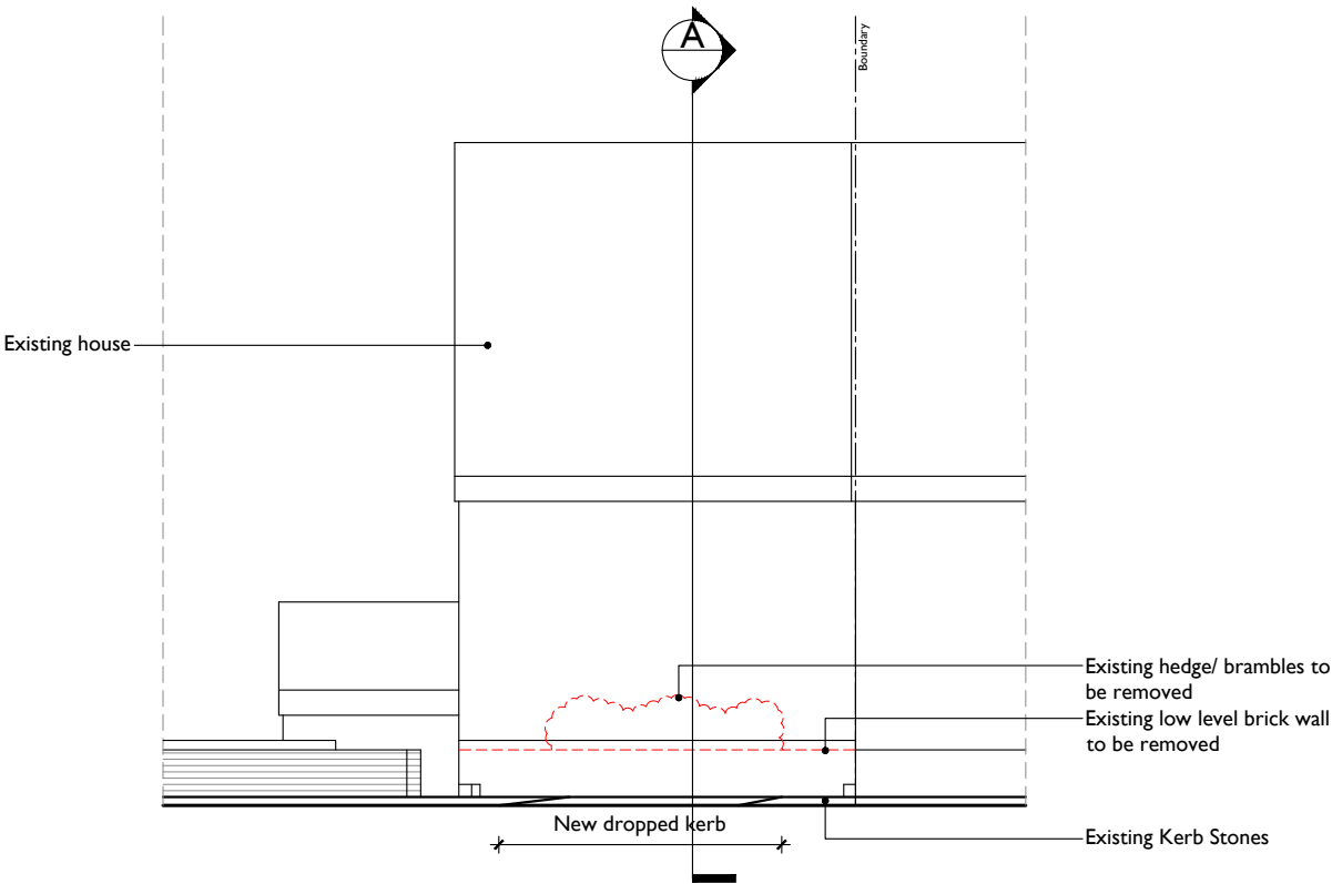
Proposed boundary wall elevation
