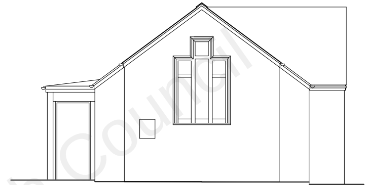
EAST ELEVATION AS EXISTING scale 1:100
