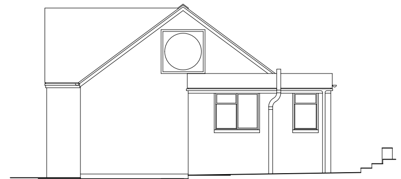
WEST ELEVATION AS EXISTING scale 1:100
