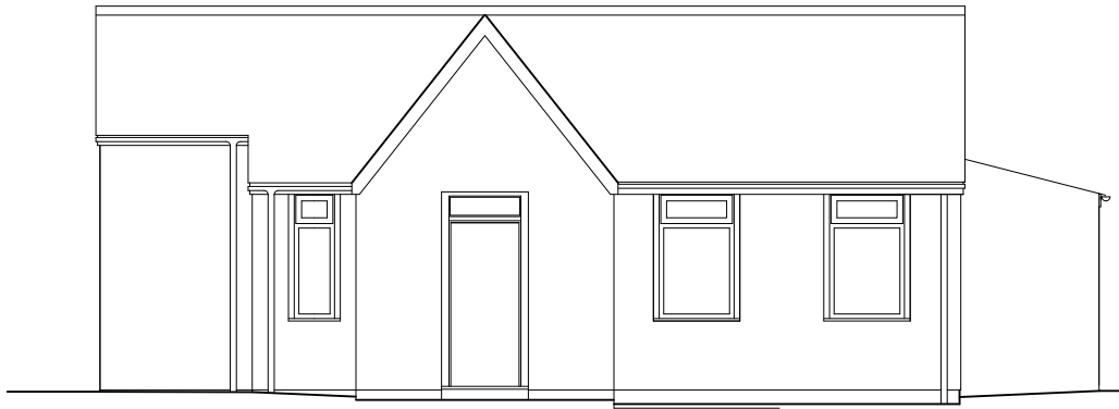
NORTH ELEVATION AS EXISTING scale 1:100
