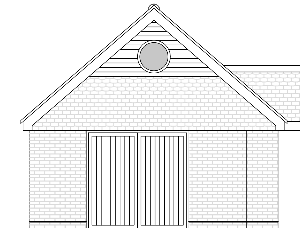
West Elevation
