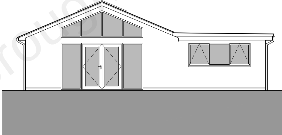
Proposed West Elevation 1:100
