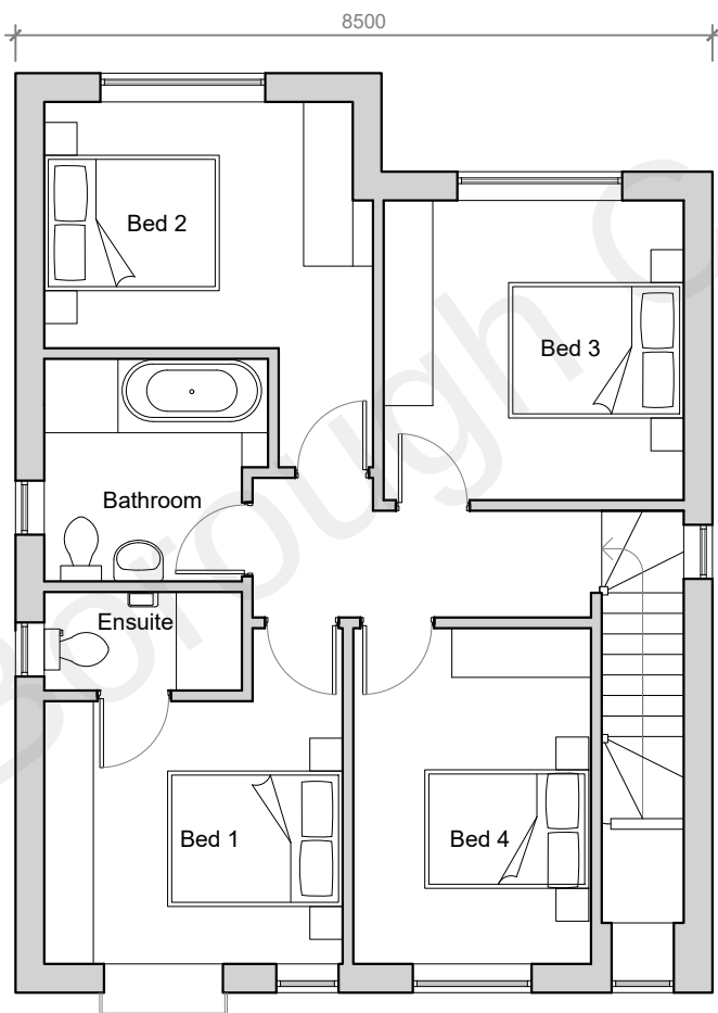
Indicative First Floor Plan
