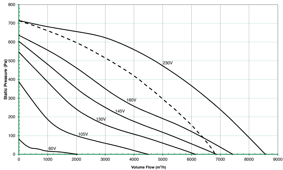
ESTOC 67-500-3 - BI101219
