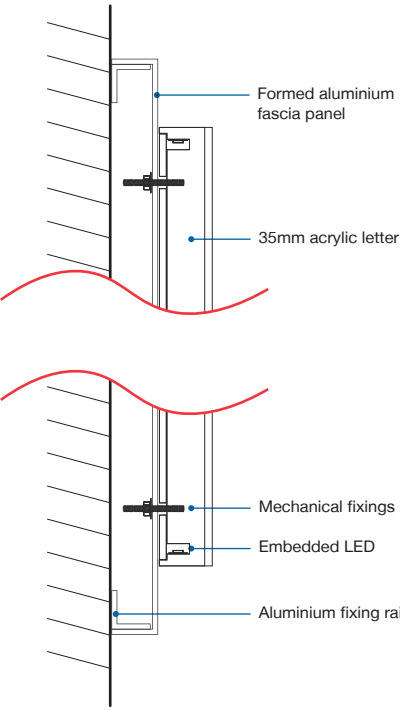
Section through - 1:5
