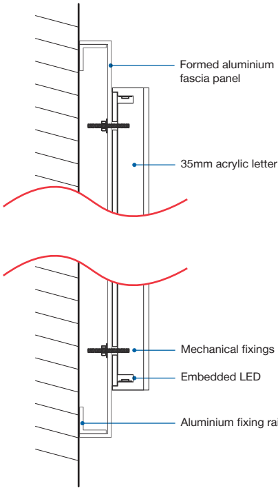
Section through - 1:5
