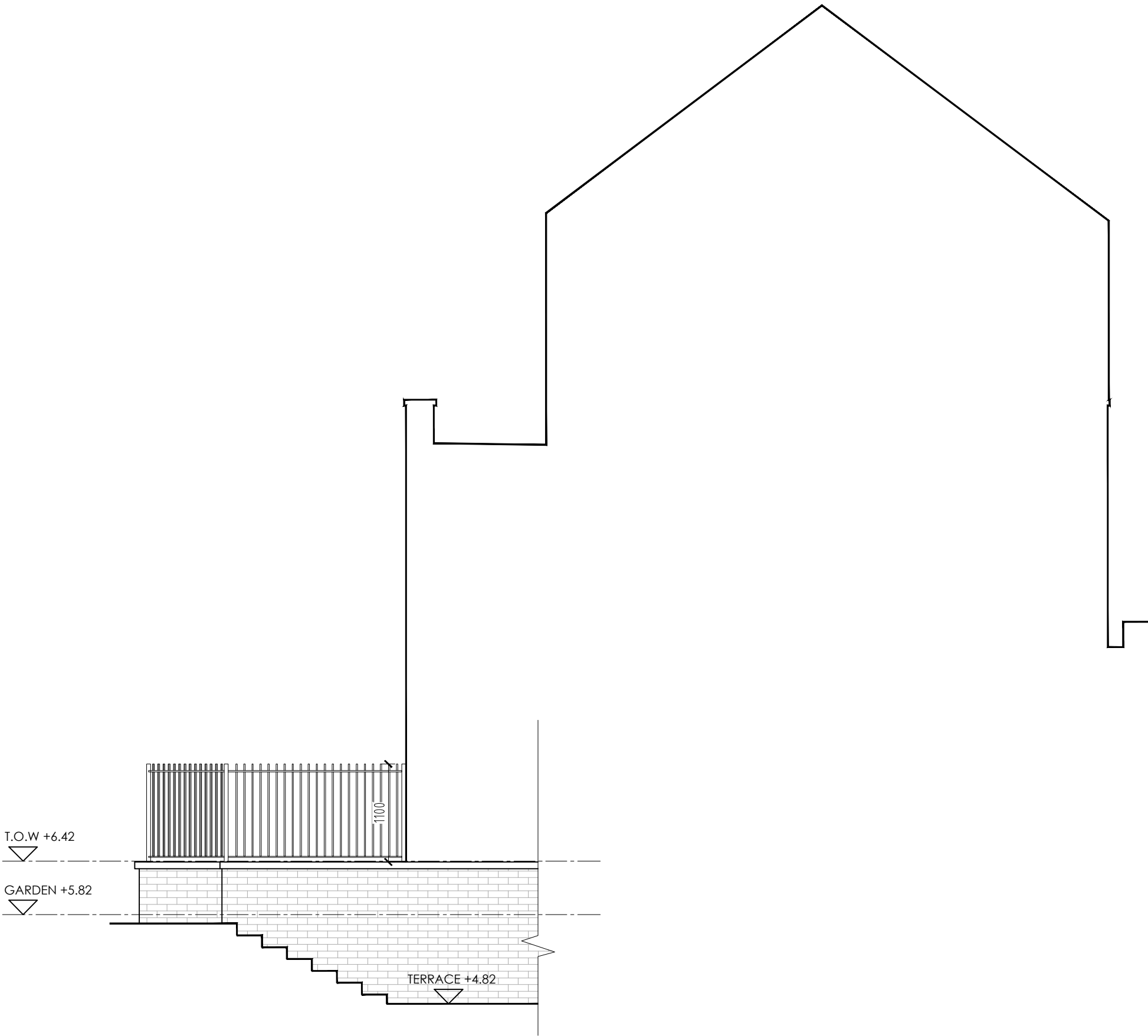
Proposed new build brick retaining wall with railing. 1.50
