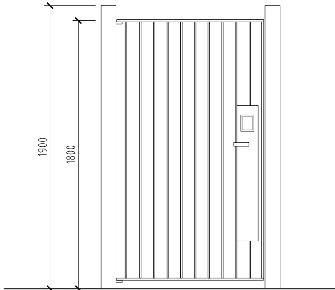
Proposed metal railing and cycle store access gate 1.25
