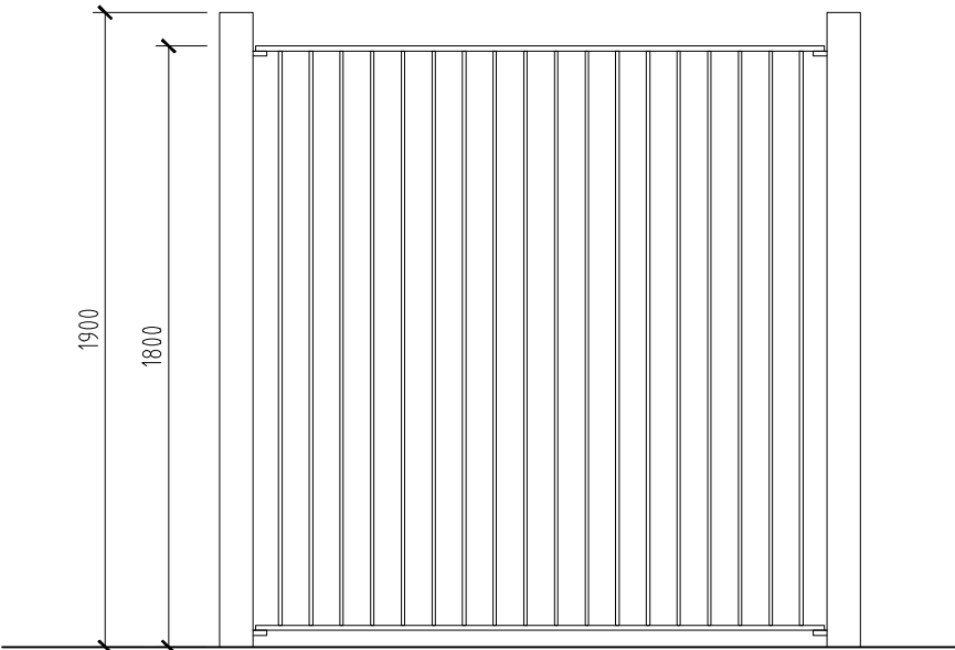
Proposed metal railing and cycle store access gate 1.25
