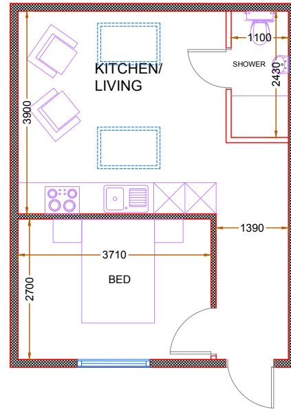
PROPOSED ANNEX FLOOR PLAN
